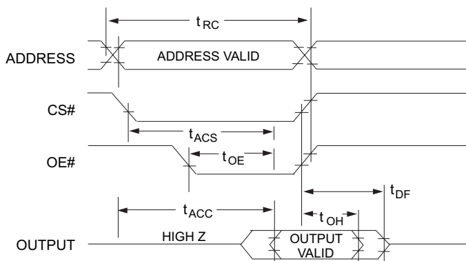
FIGURE 3 – READ WAVEFORMS
