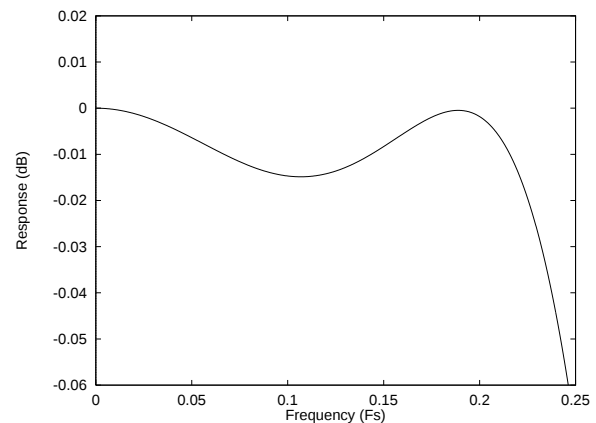
Figure 40 DAC Digital Filter Ripple –Type 2
