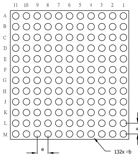
Bottom View
