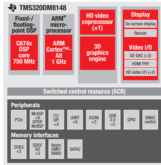
▲ DM8148 processor block diagram
