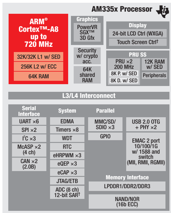
▲ AM335x ARM MPU block diagram
