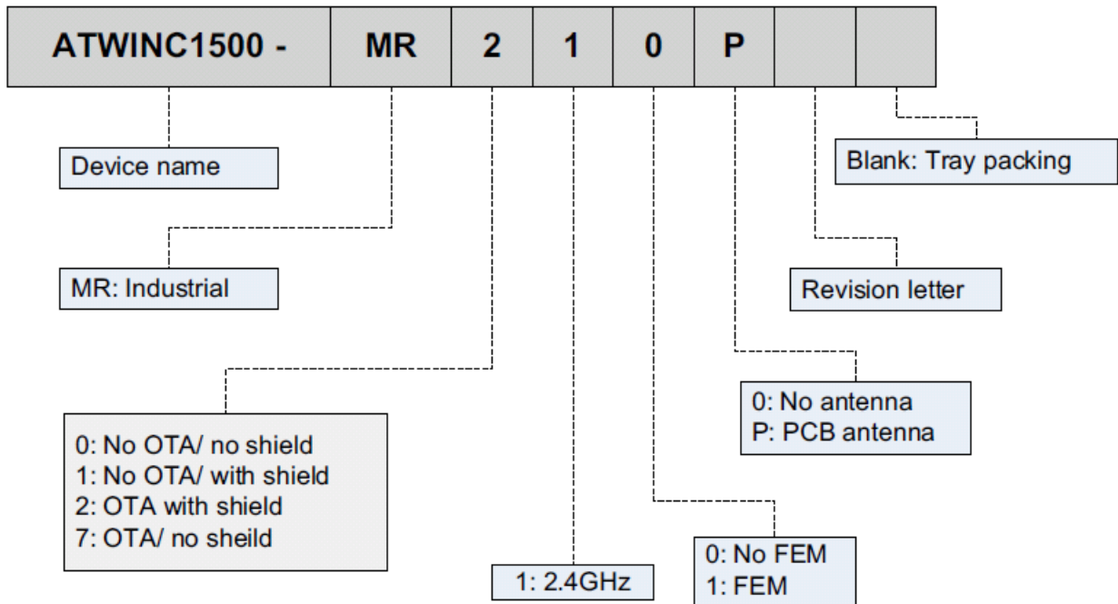
Figure 1-1. Marking Information
