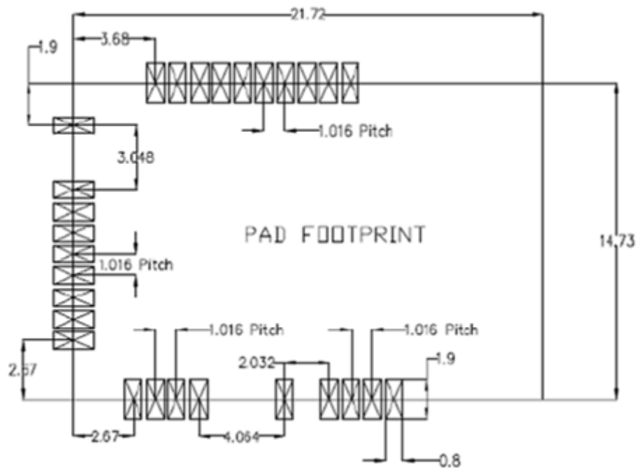
Figure 11-1. Footprint Drawing
