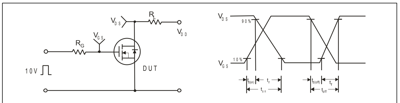
Fig.13 Resistive Switching Test Circuit &amp; Waveform
