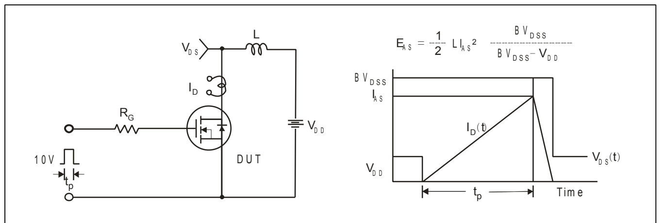
Fig.14 Uncamped Inductive Switching Test Circuit &amp; Waveform
