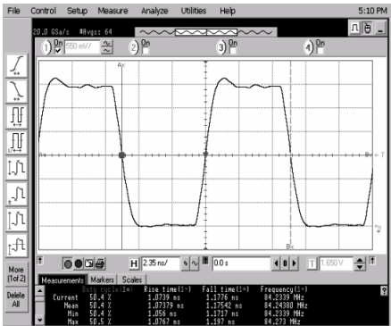
5027×D, V_{DD} = 3.3V , f_{OUT} = 85MHz , C_L = 15pF , T_a = 25^{\circ}C
