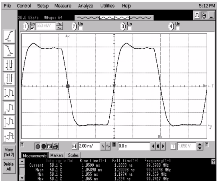
5027×D, V_{DD} = 3.3V , f_{OUT} = 100MHz , C_L = 15pF , T_a = 25^{\circ}C
