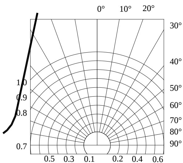
RADIATION DIAGRAM
