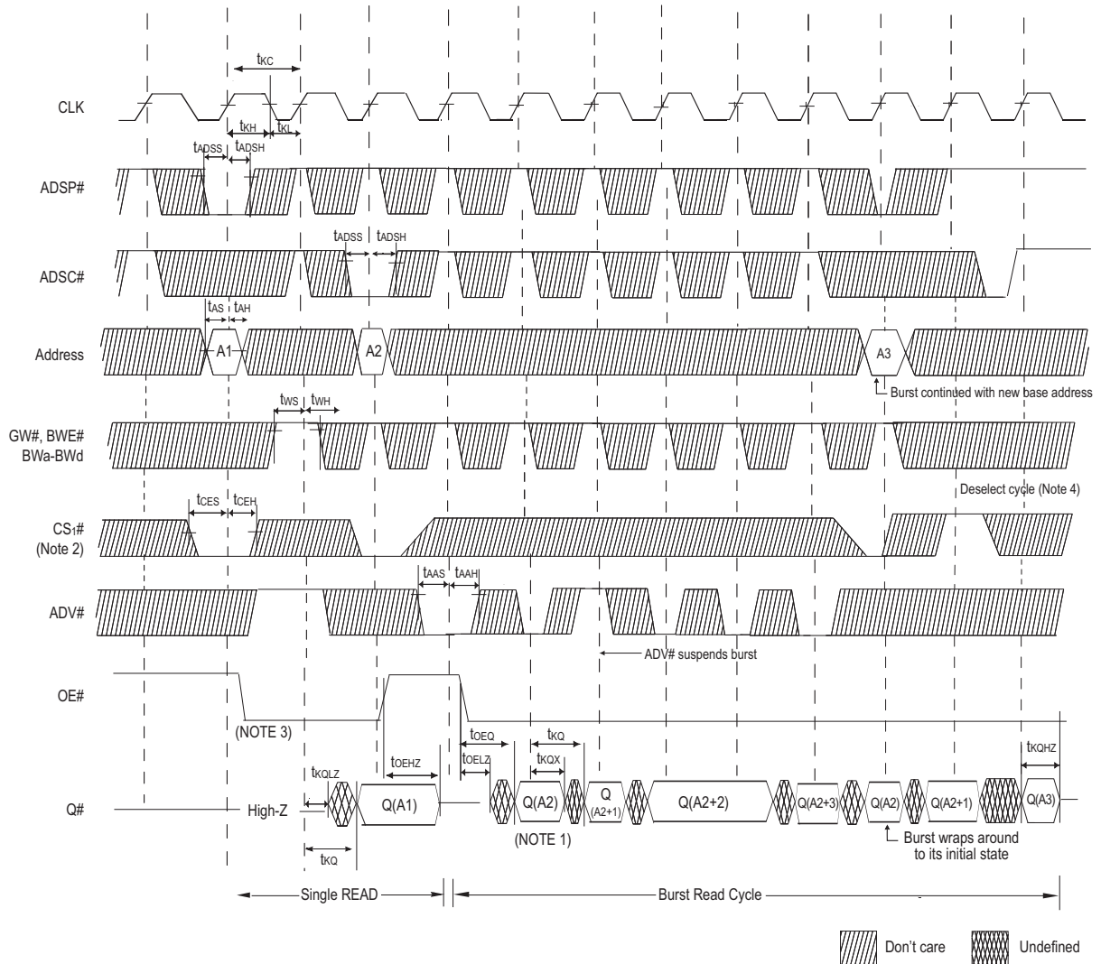
FIGURE 2 – READ TIMING 3
