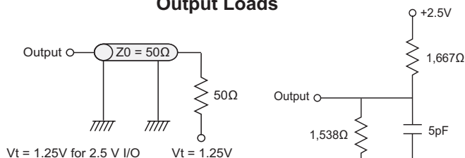
AC Output Load Equivalent
