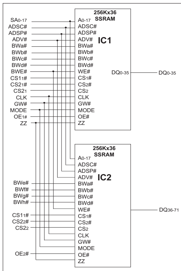
FIGURE 1 – BLOCK DIAGRAM
