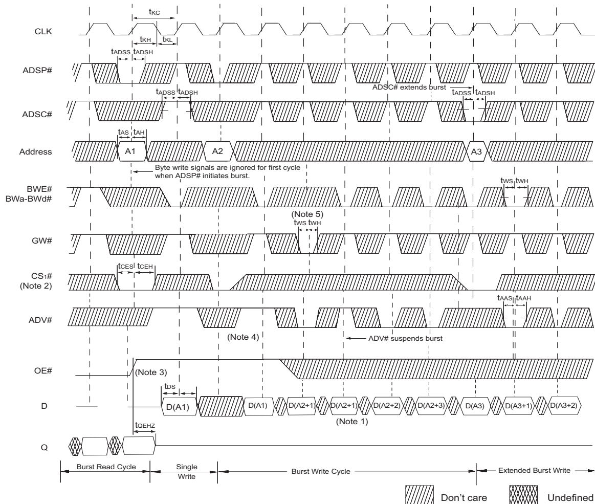
FIGURE 3 – WRITE TIMING
