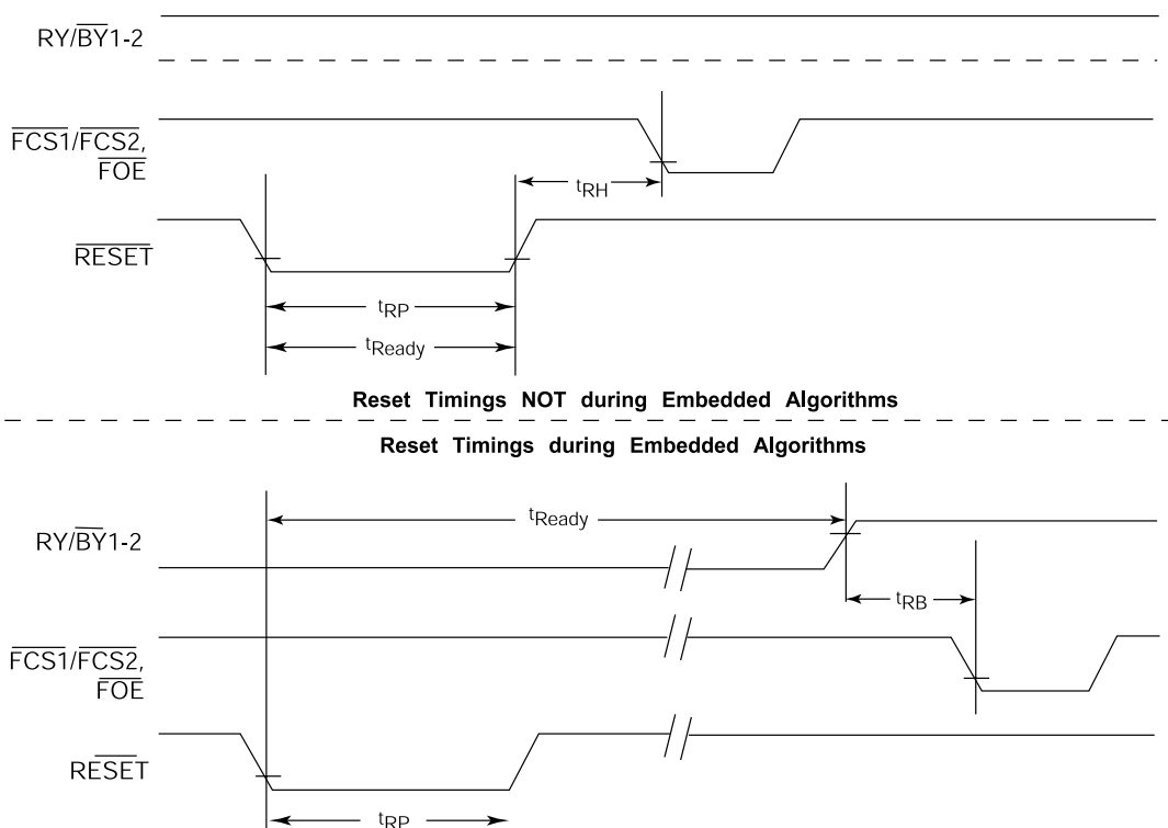
FIG. 19 HARDWARE RESET ( \overline{\text{RST}} )
