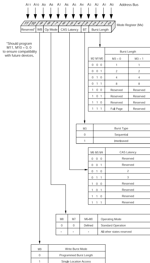
FIG. 3 MODE REGISTER DEFINITION
