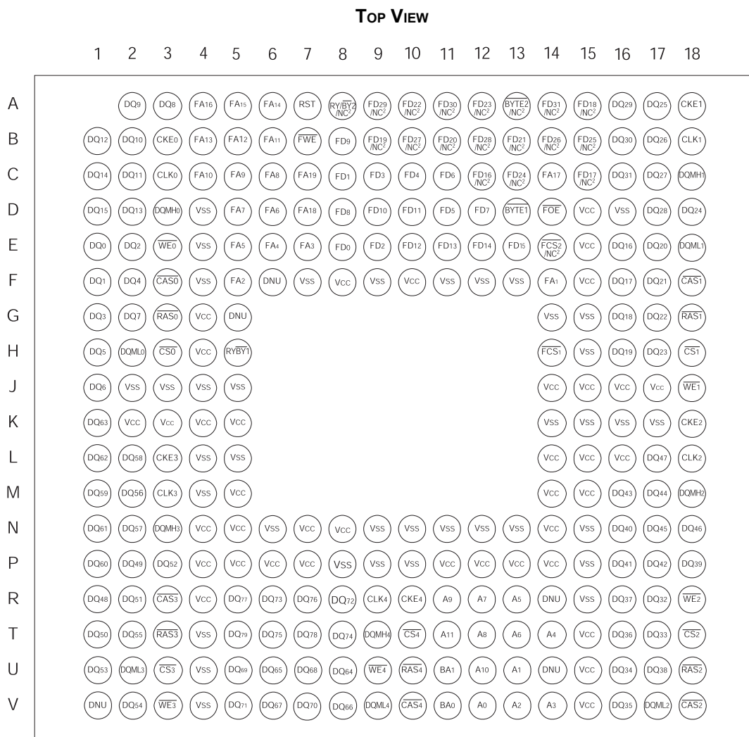
FIG. 1 PIN CONFIGURATION
