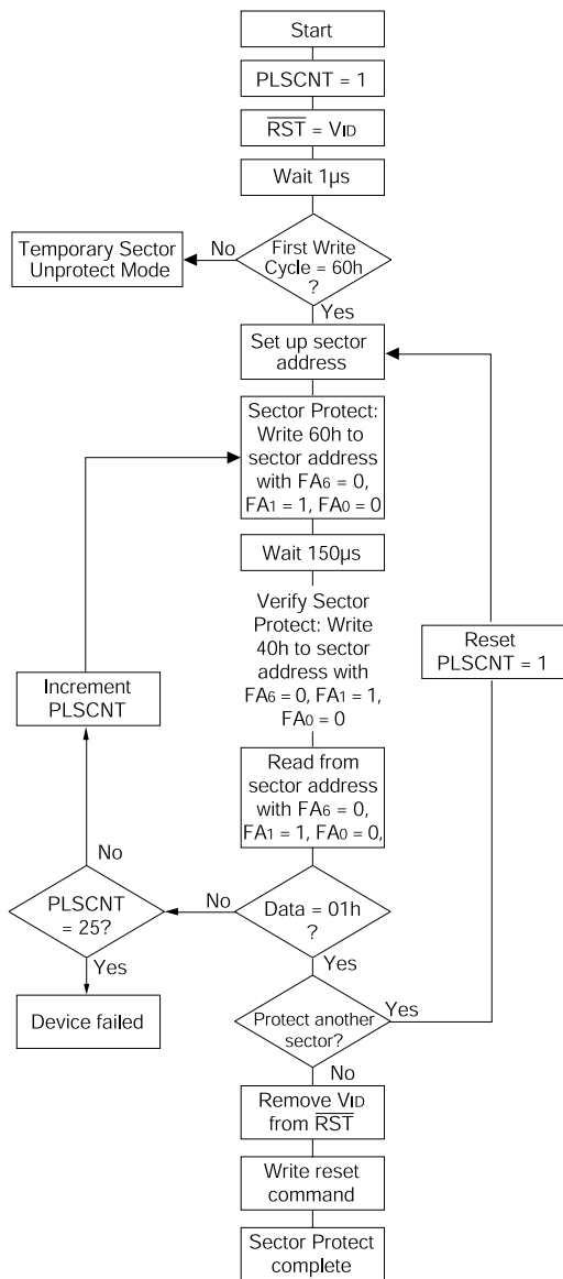
FIG. 5 SECTOR PROTECT/UNPROTECT ALGORITHMS
