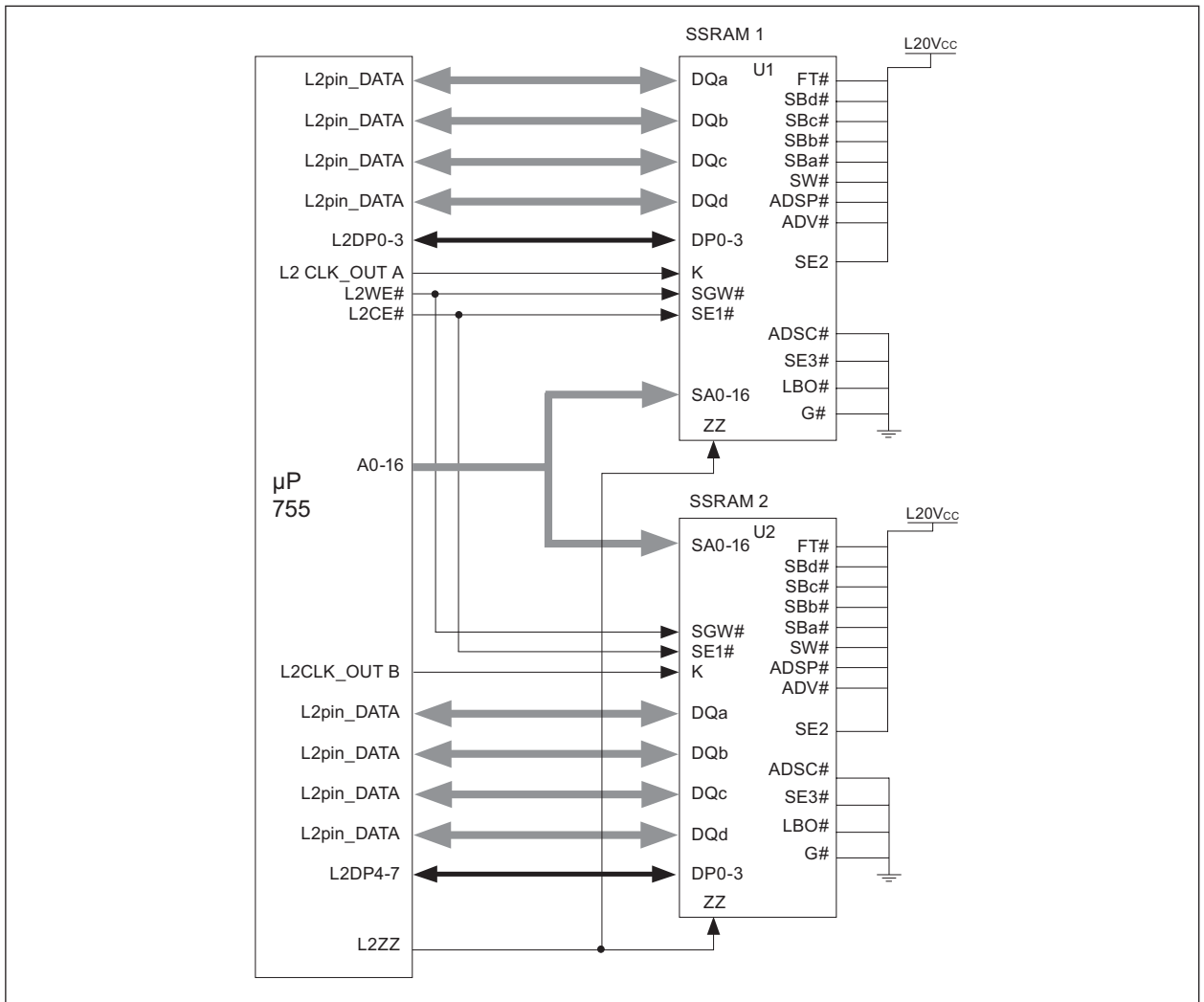
FIGURE 3 – BLOCK DIAGRAM, L2 INTERCONNECT
