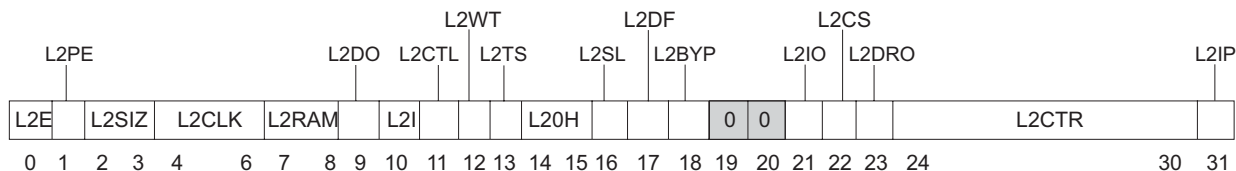
FIGURE 5 – L2 CACHE CONTROL REGISTER (L2CR)
