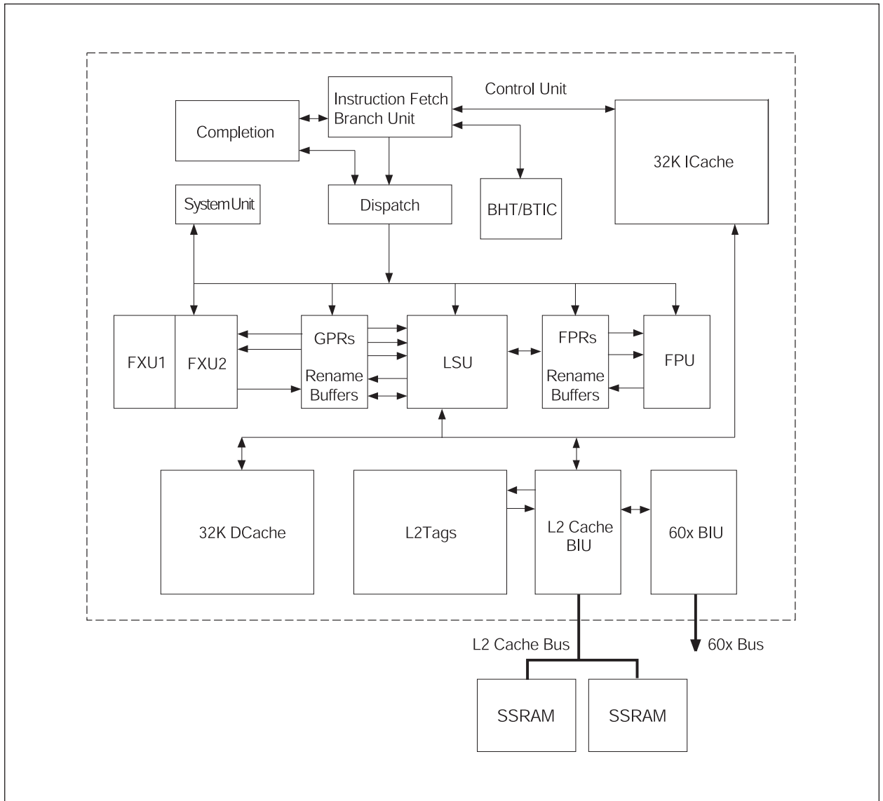
FIGURE 2 – BLOCK DIAGRAM
