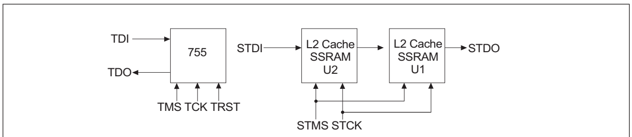
FIGURE 4 – BLOCK DIAGRAM, L2 INTERCONNECT
