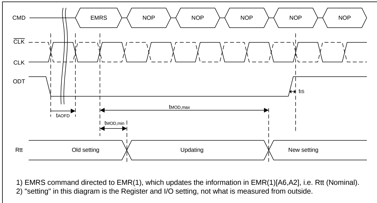
Figure 10 – ODT updates delay timing - tMOD
