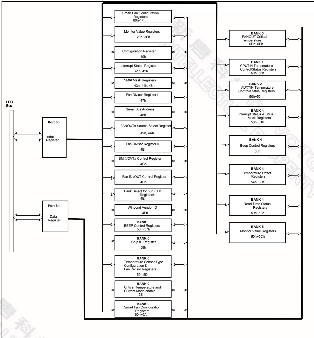
Figure 8-1 LPC Bus' Reads from / Writes to Internal Registers
