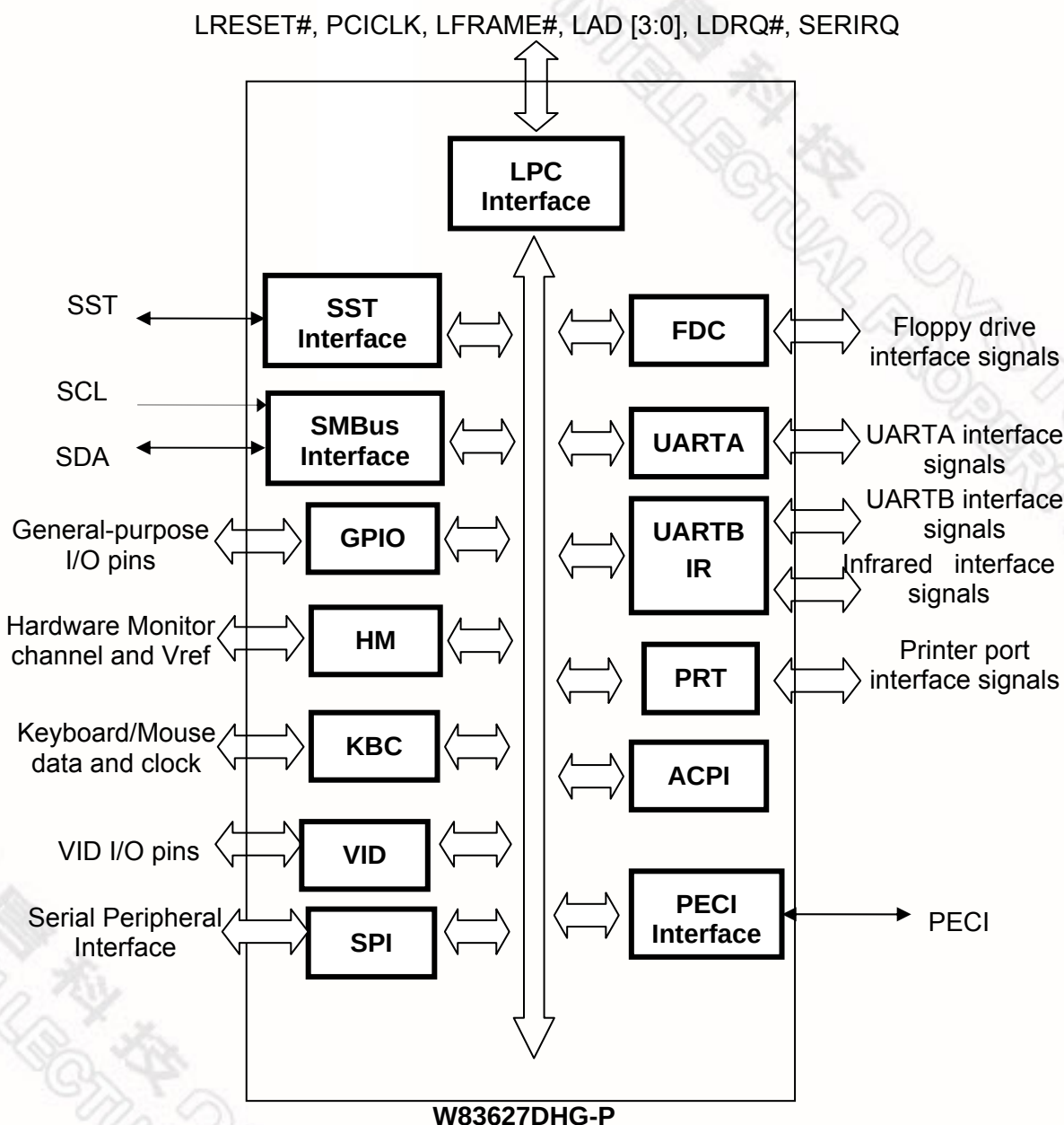
Figure 3-1 W83627DHG-P Block Diagram
