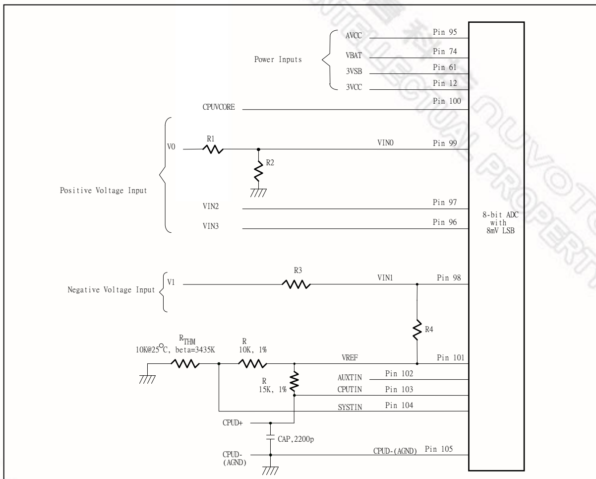
Figure 8-4 Analog Inputs and Application Circuit of the W83627DHG-P
