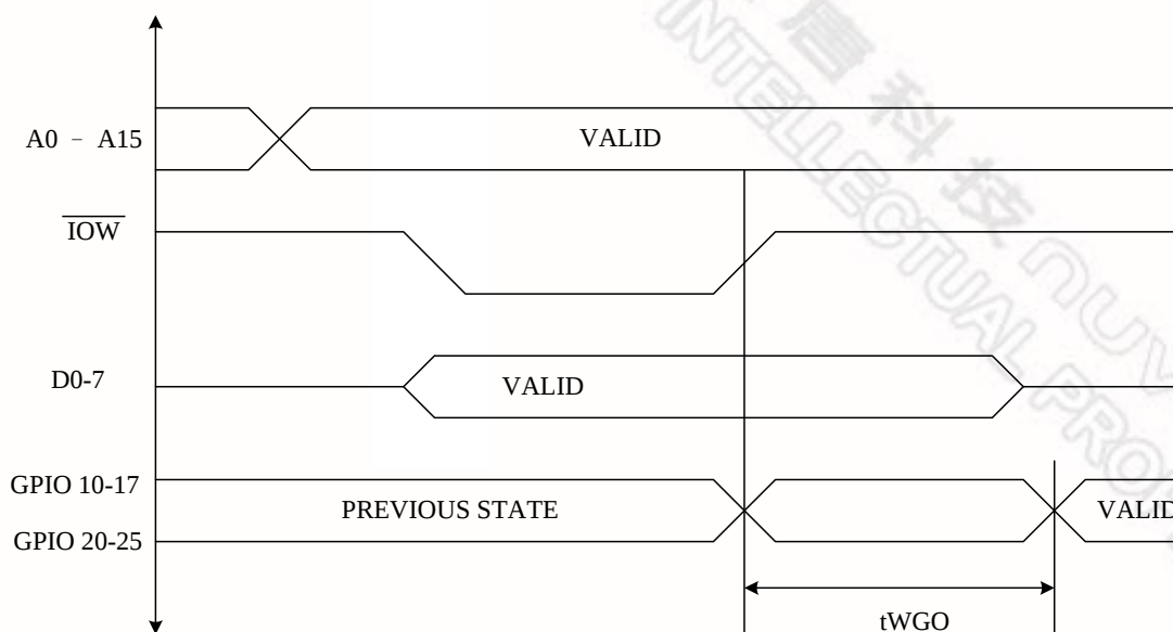
GPIO Write Timing diagram
