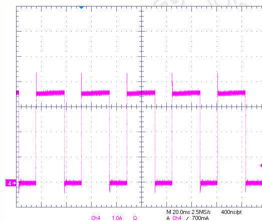
VIN=1.8V, VCNTL=5V, VOUT=0.9V, VOUT short to VIN
