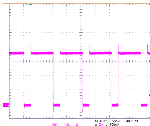
VIN=1.5V, VCNTL=5V, VOUT=0.75V, VOUT short to GND
