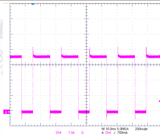
VIN=1.8V, VCNTL=5V, VOUT=0.9V, VOUT short to GND
