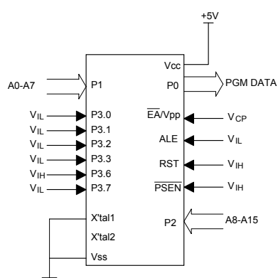
Programming Verification
