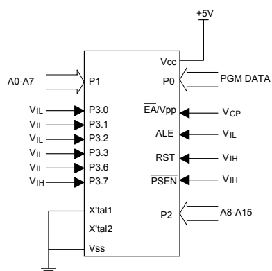
Programming Configuration
