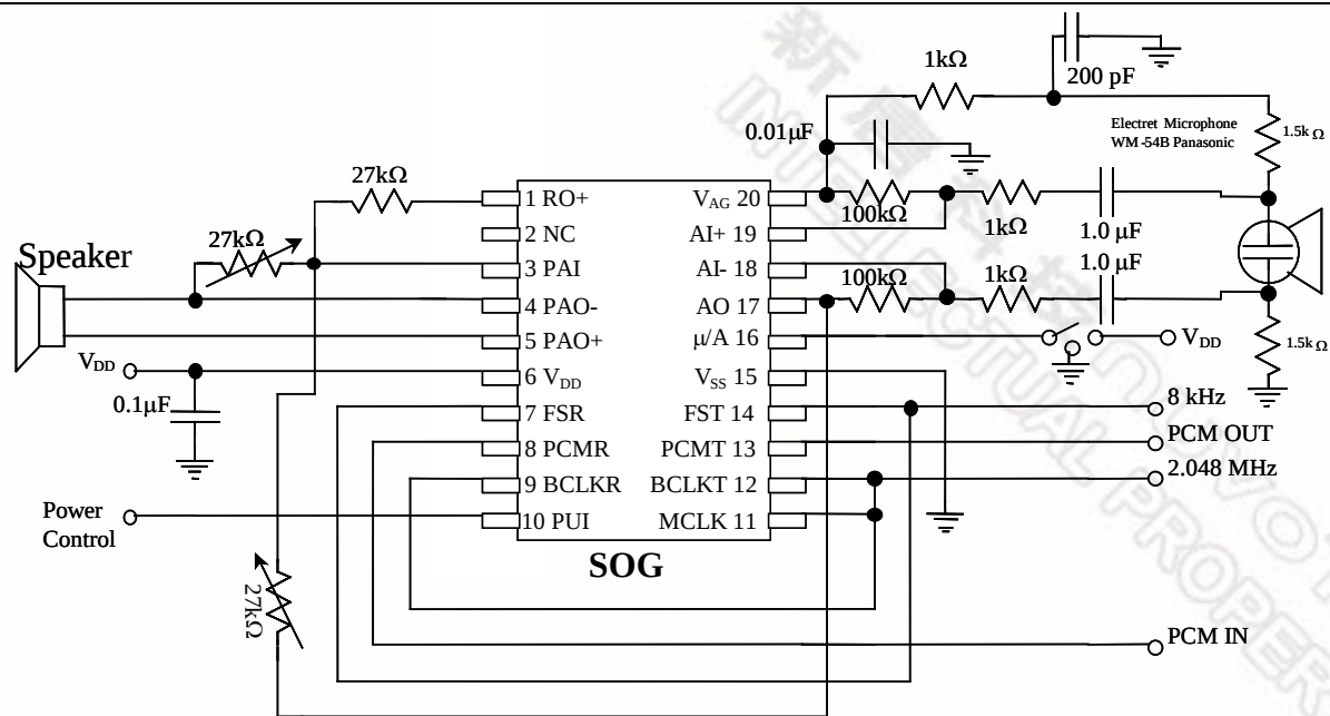
Figure 11.3 Handset Interface
