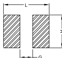
Recommend PC Board Pattern
