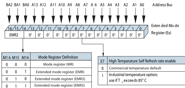
FIGURE 8 – EXTENDED MODE REGISTER 2 (EMR2) DEFINITION
