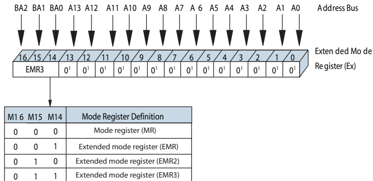
FIGURE 9 – EXTENDED MODE REGISTER 3 (EMR3) DEFINITION
