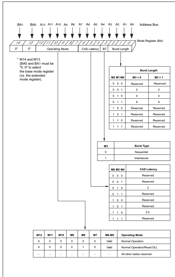
FIGURE 3 – MODE REGISTER DEFINITION
