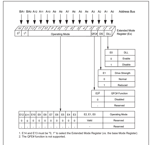
FIGURE 5 – EXTENDED MODE REGISTER DEFINITION
