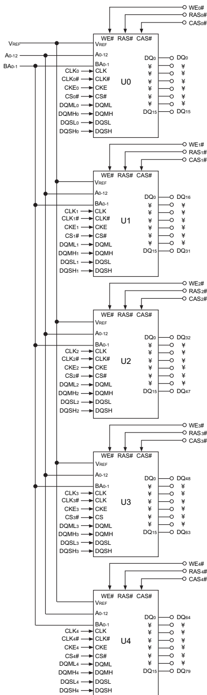
FIGURE 2 – FUNCTIONAL BLOCK DIAGRAM
