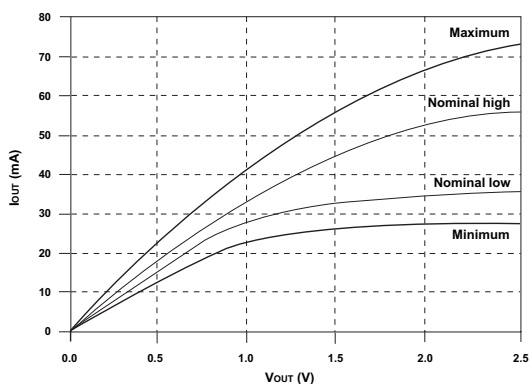
FIGURE C – PULL-DOWN CHARACTERISTICS
