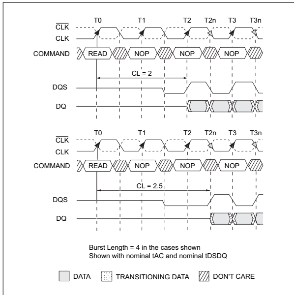
FIGURE 4 – CAS LATENCY
