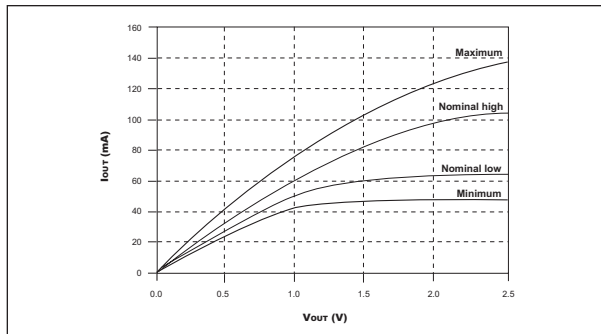
FIGURE A – PULL-DOWN CHARACTERISTICS
