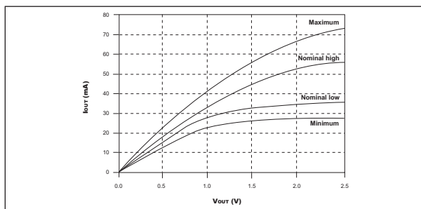
FIGURE C – PULL-DOWN CHARACTERISTICS
