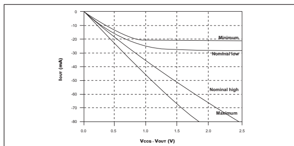
FIGURE D – PULL-UP CHARACTERISTICS
