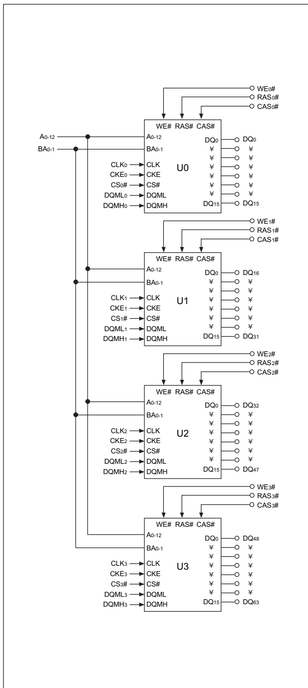
FIGURE 2 – FUNCTIONAL BLOCK DIAGRAM
