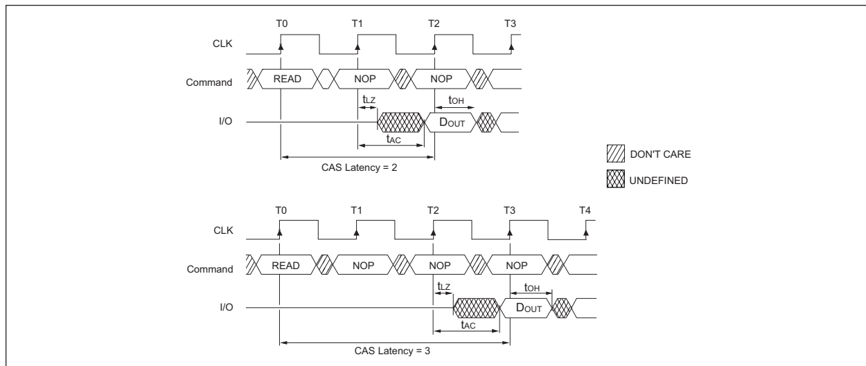
FIGURE. 4 – CAS LATENCY
