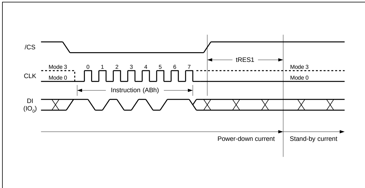
Figure 20. Release Power-down Instruction Sequence
