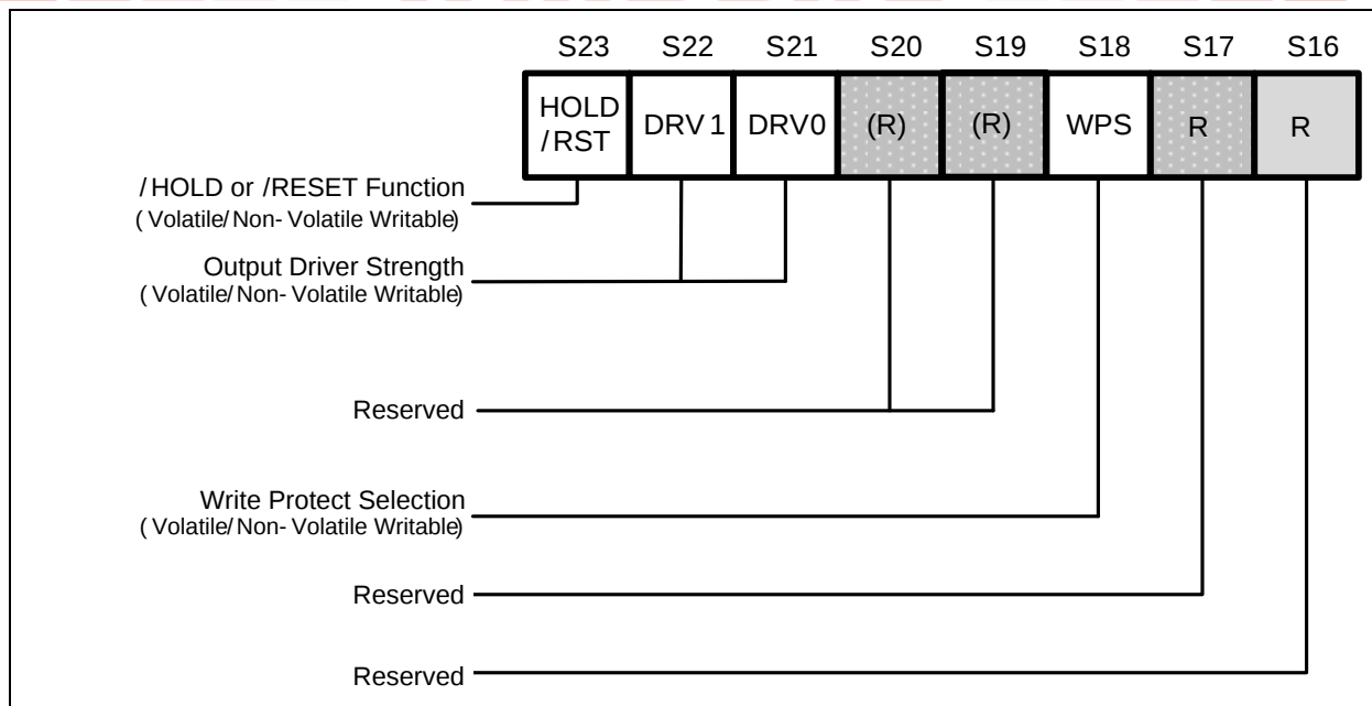
Figure 4c. Status Register-3
