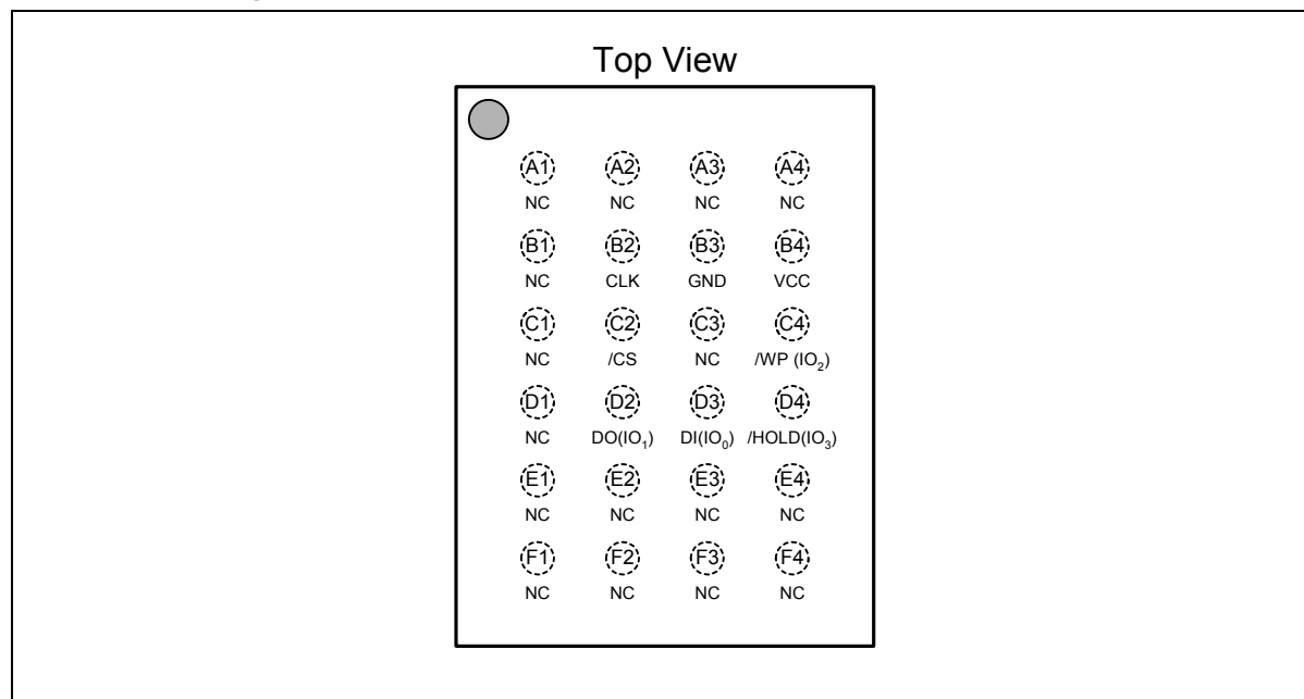
Figure 1e. W25Q64CV Ball Assignments, 24-ball TFBGA 8x6-mm (Package Code TC)
