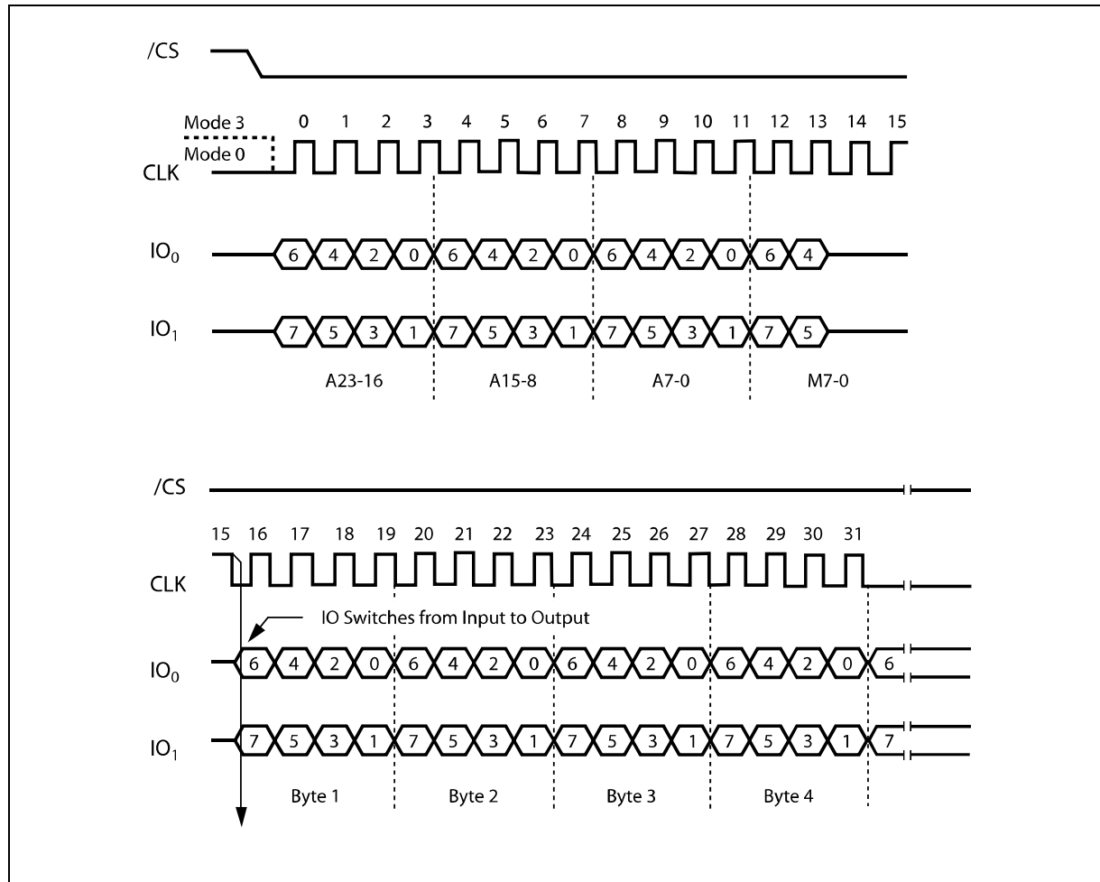
Figure 12b. Fast Read Dual Input/Output Instruction Sequence Diagram (M7-0 = A7h)
