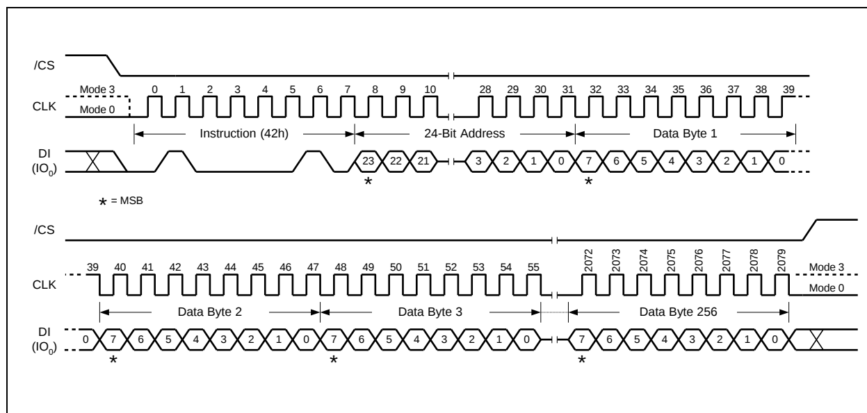
Figure 36. Program Security Registers Instruction Sequence
