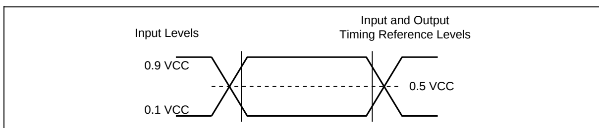
Figure 40. AC Measurement I/O Waveform
