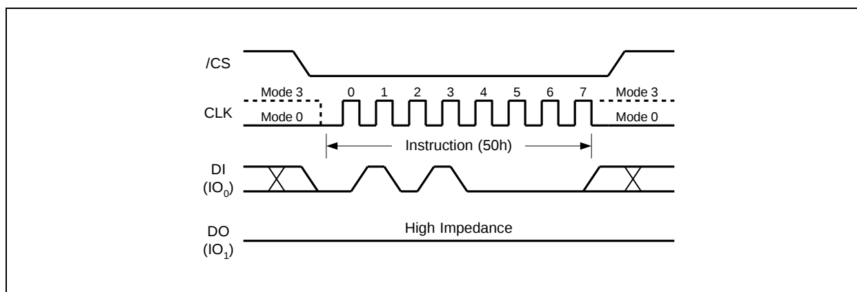
Figure 5. Write Enable for Volatile Status Register Instruction Sequence Diagram
