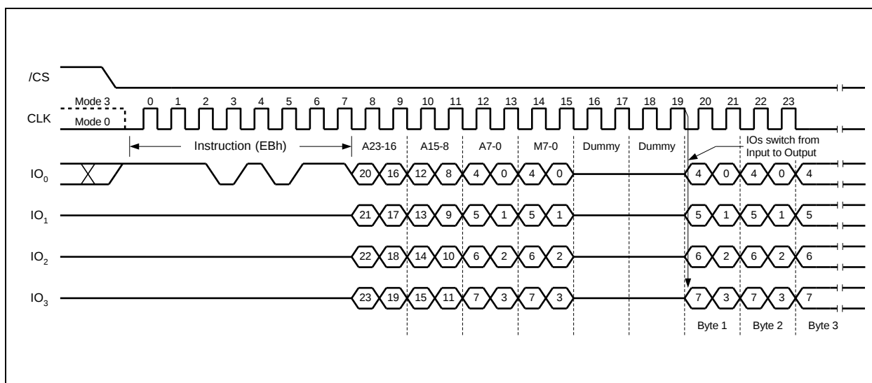
Figure 14a. Fast Read Quad I/O Instruction Sequence (Initial instruction or previous M5-4 ≠ 10)
