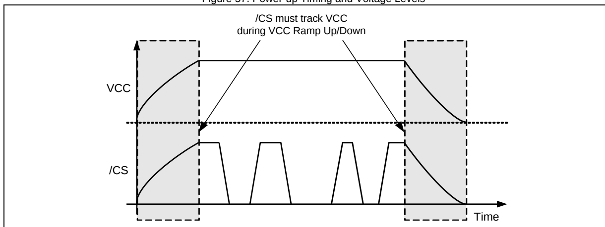
Figure 57a. Power-up, Power-Down Requirement
