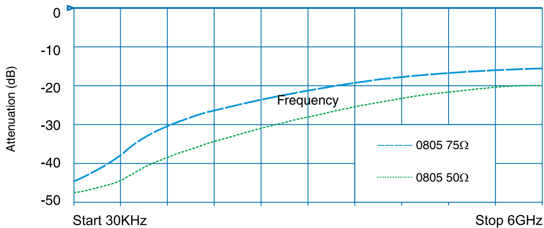
W0805HF Frequency Performance
