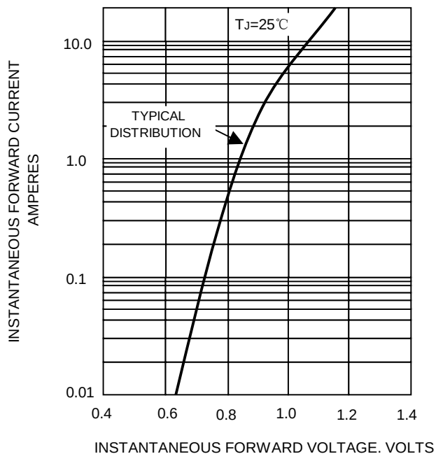
FIG.3-TYPICAL FORWARD CHARACTERISTICS
