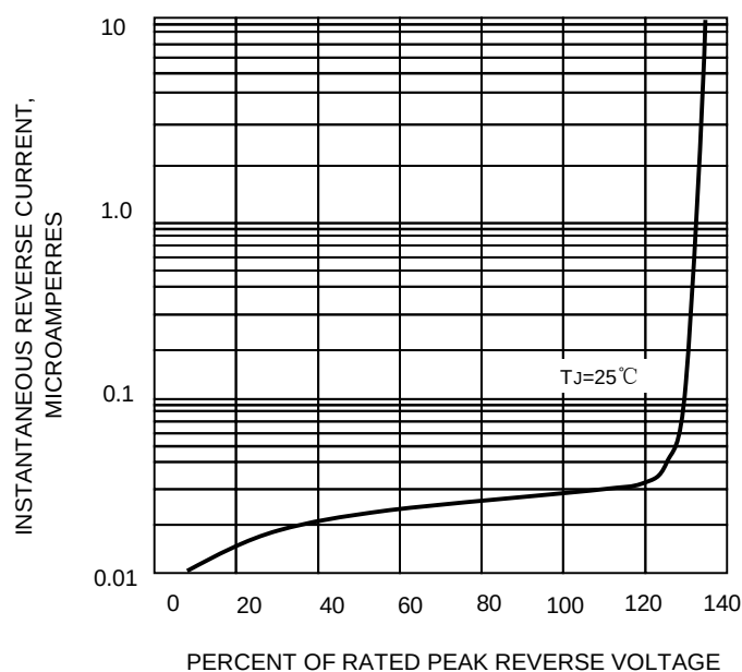
FIG.4-TYPIACL REVERSE CHARACTERISTICS
