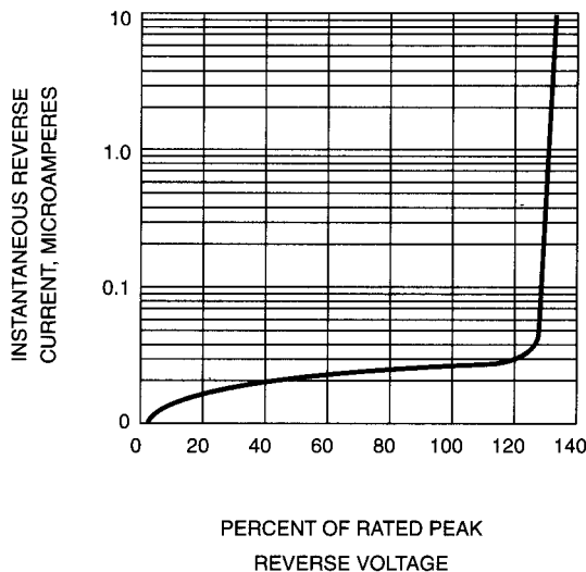
FIG. 4-TYPICAL REVERSE CHARACTERISTICS
