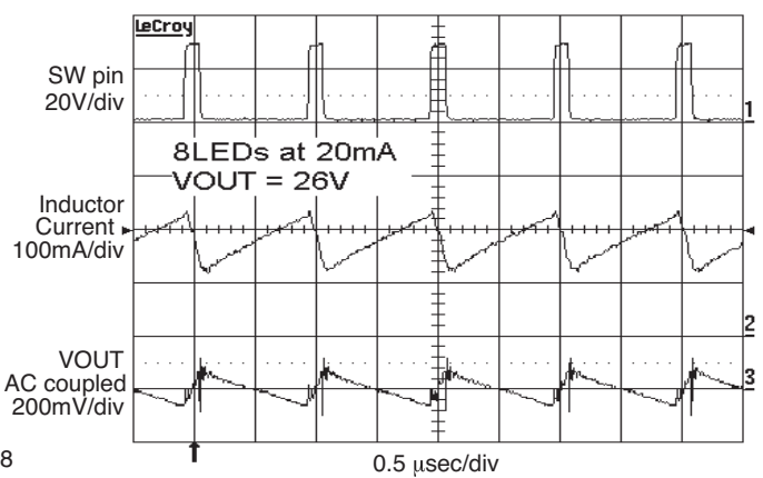
Figure 9. Switching Waveforms
