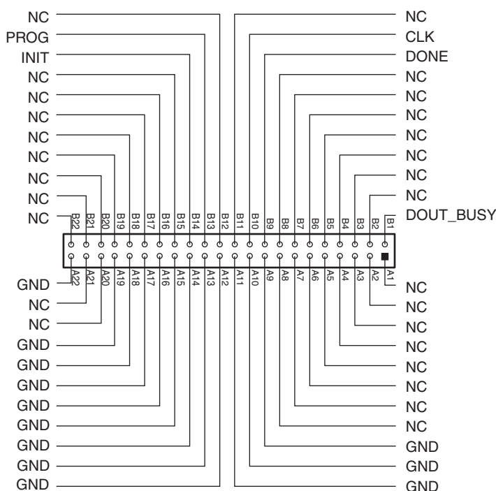
Figure 7: Downstream Interface Connector (44-Pin Male)
