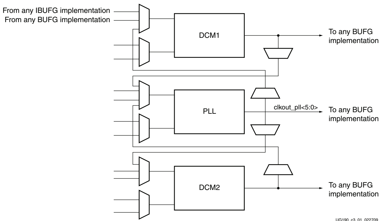
Figure 3-1: Block Diagram of the Virtex-5 FPGA CMT
