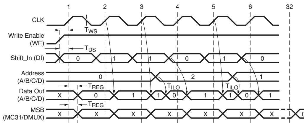
Figure 5-30: Slice SRL Timing Characteristics
