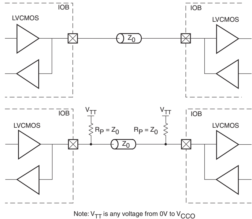
Figure 6-30: LVC MOS Bidirectional Termination
