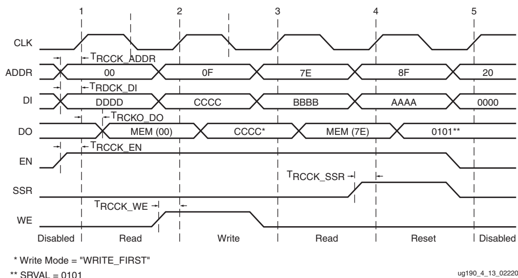
Figure 4-14: Block RAM Timing Diagram
