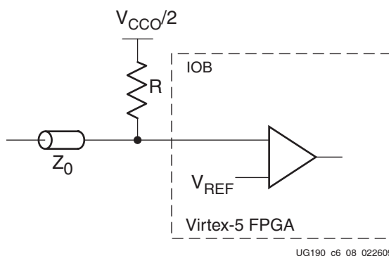
Figure 6-10: Input Termination to V_{CCO}/2 without DCI
