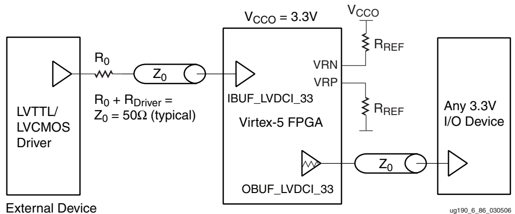
Figure 6-92: Connecting LVTTTL or LVCMOS Using the LVDCI_33 Standard
