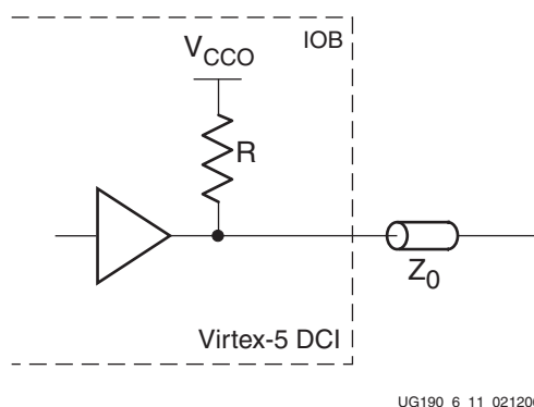
Figure 6-13: Driver with Termination to V_{CCO} Using DCI Single Termination
