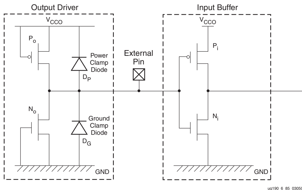
Figure 6-91: Virtex-5 FPGA I/O: 3-State Output Driver
