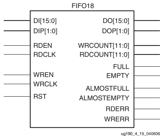
Figure 4-19: FIFO18 Primitive
