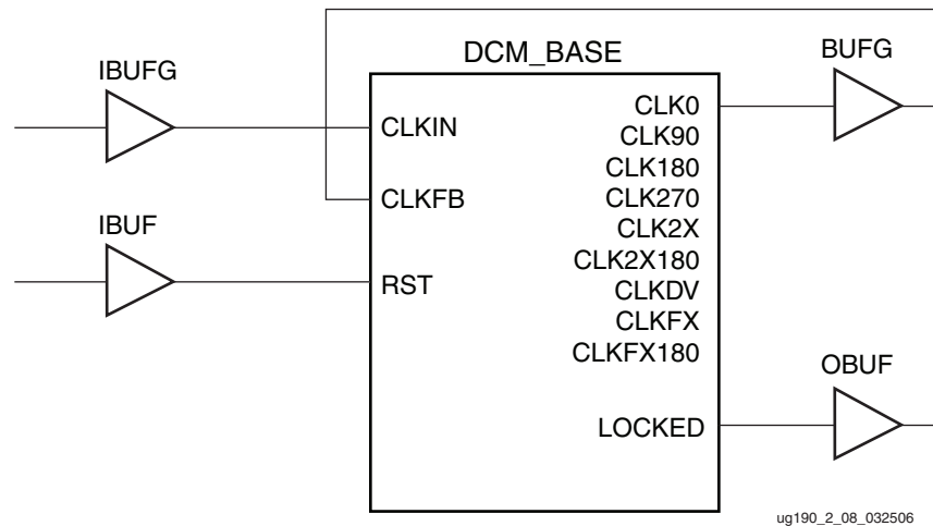
Figure 2-8: Standard Usage
