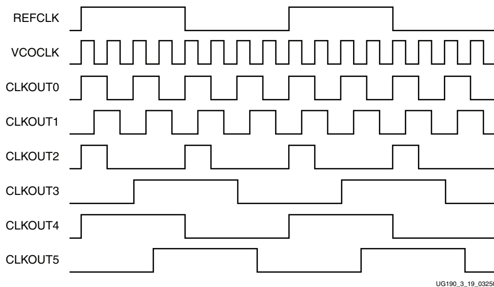
Figure 3-16: Example Waveform
