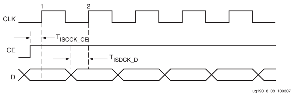
Figure 8-8: ISERDES Input Data Timing Diagram
