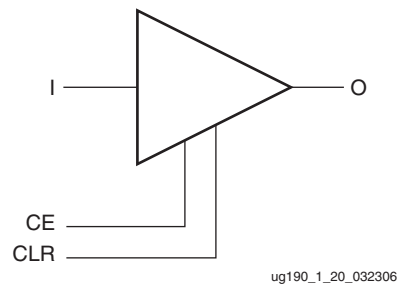
Figure 1-20: BUFR Primitive
