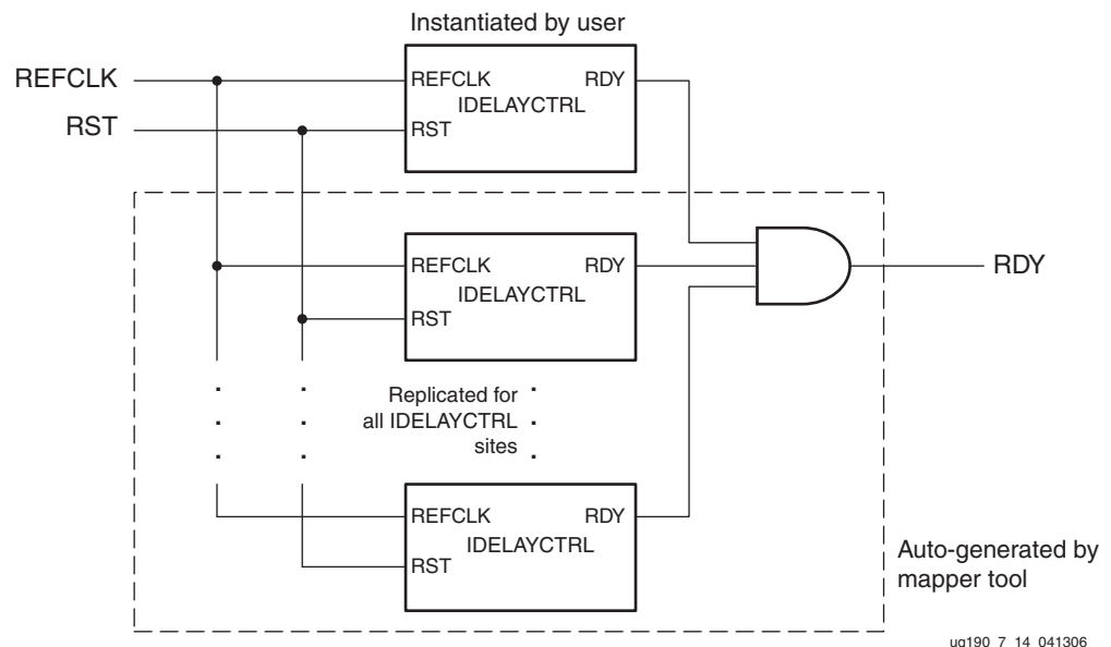
Figure 7-19: Instantiate IDELAYCTRL Without LOC Constraints - RDY Connected
