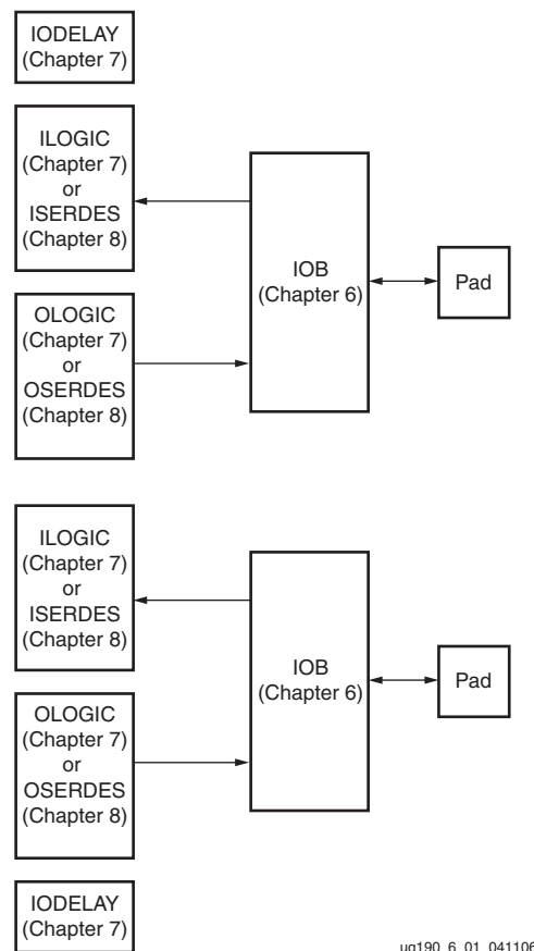
Figure 6-1: Virtex-5 FPGA I/O Tile
