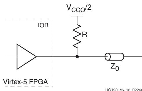
Figure 6-14: Driver with Termination to V_{CCO}/2 without DCI
