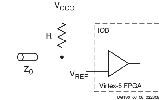
Figure 6-8: Input Termination to V_{CCO} without DCI
