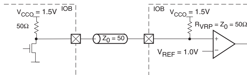
Figure 6-39: GTLP_DCI Internal Parallel Driver and Receiver Termination
