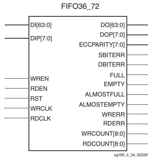
Figure 4-30: FIFO36_72: FIFO ECC Primitive
