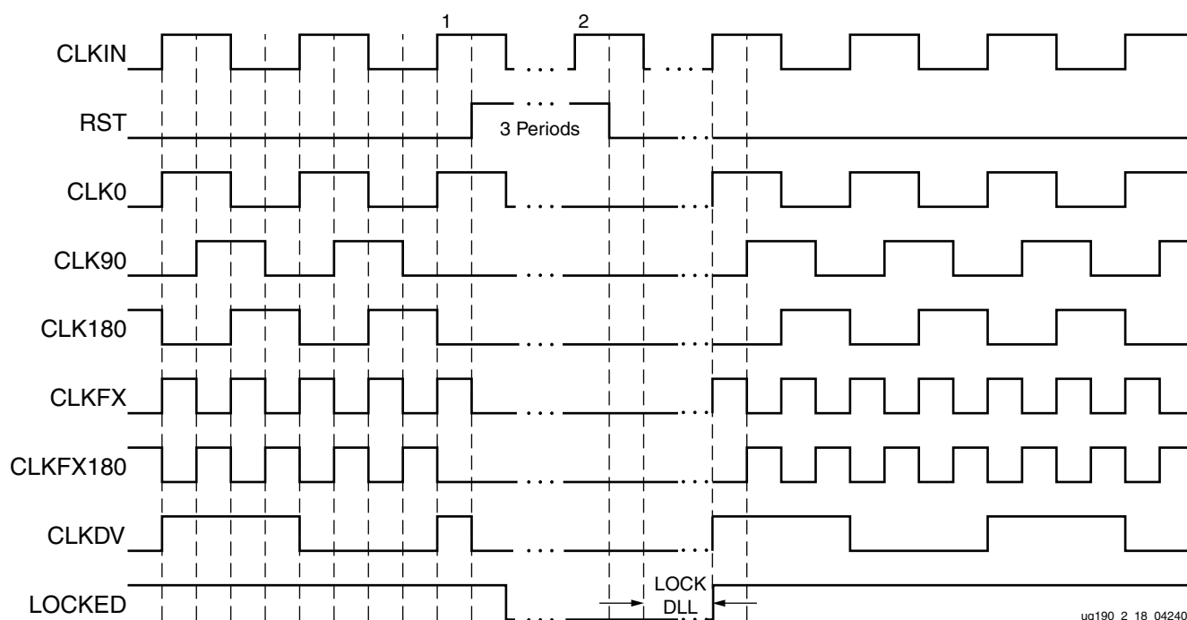
Figure 2-17: RESET/LOCK Example
