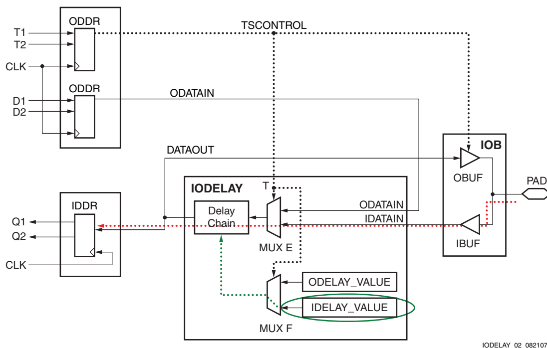
Figure 7-11: IOB and IODELAY in Input Mode when 3-state is Disabled
