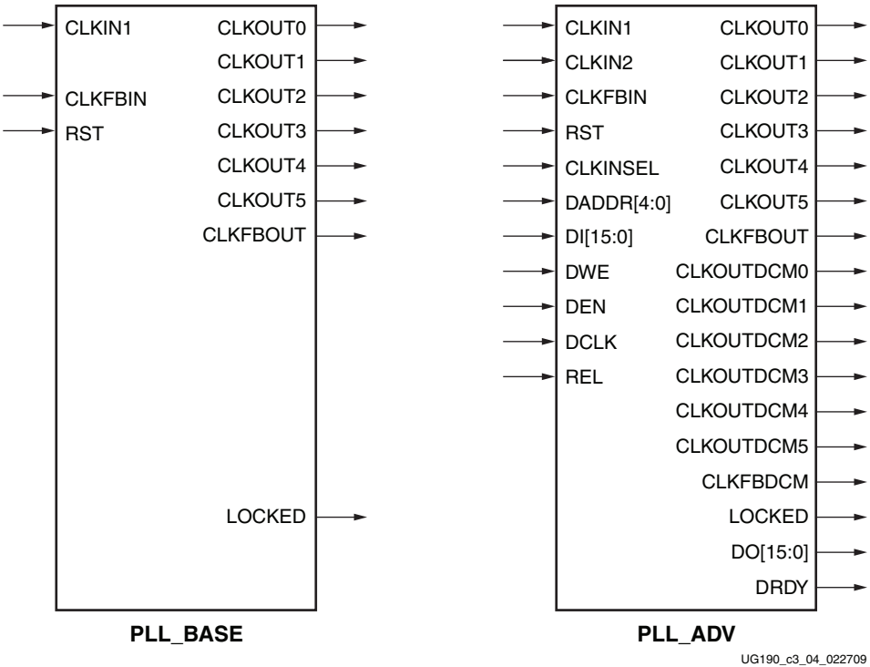
Figure 3-4: PLL Primitives
