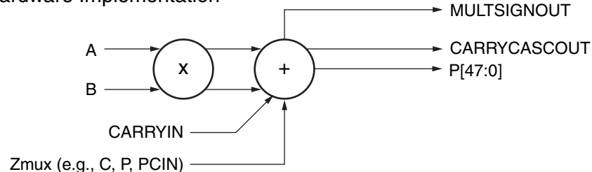
Figure A-5: MACC Software and Hardware Models
