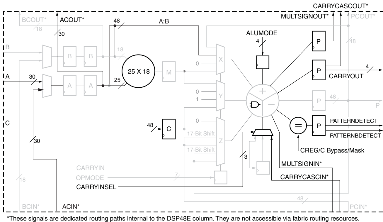
Figure 1-2: New Features in the DSP48E Slice vs. the DSP48 Slice
