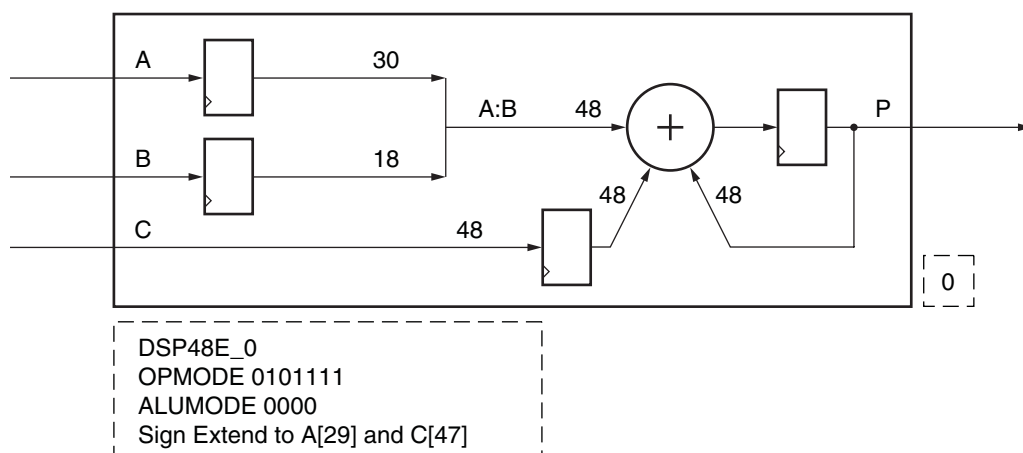
Figure 4-19: Two 48-Bit Add Accumulate Function
