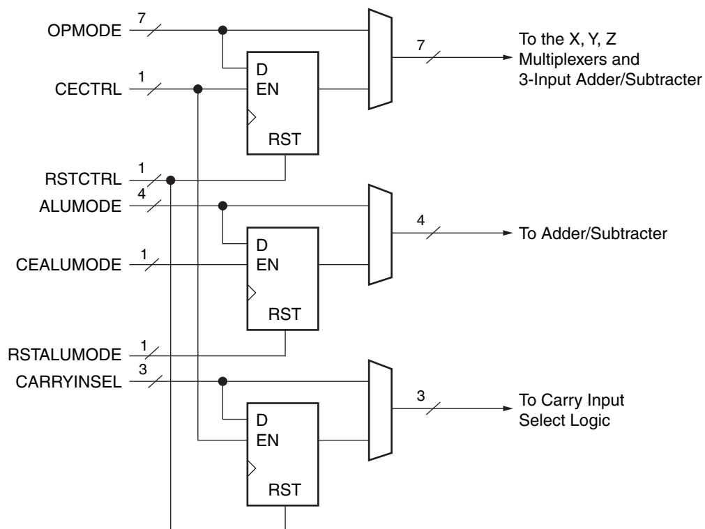
Figure 1-9: OPMODE, ALUMODE, and CARRYINSEL Port Logic
