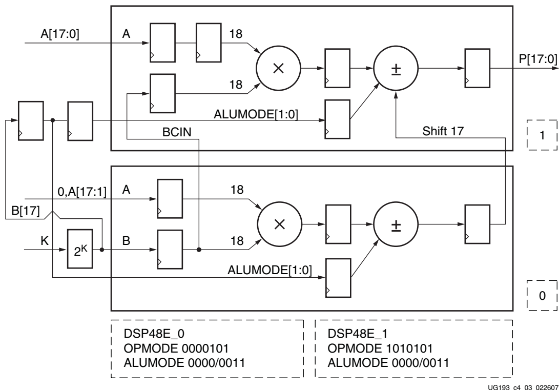
Figure 4-3: 18-Bit Barrel Shifter
