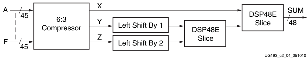
Figure 2-4: Six-Input Adder
