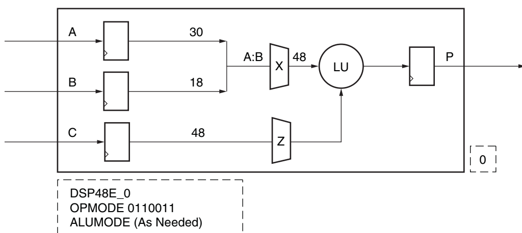
Figure 4-1: Two-Input 48-Bit Logic Function
