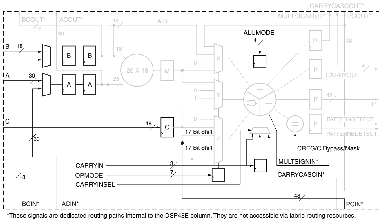
Figure 1-6: Input Ports in DSP48E Slice
