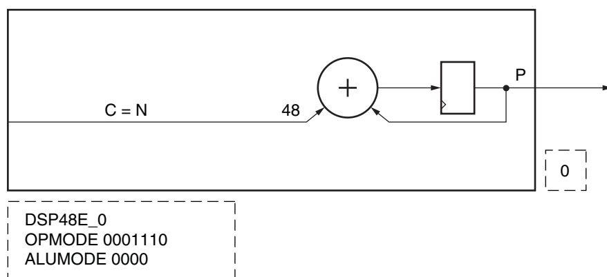
Figure 4-4: 48-Bit Counter
