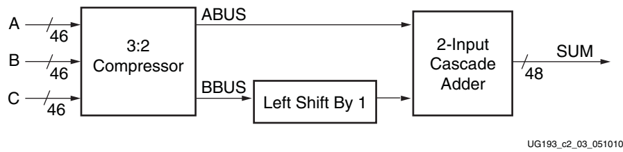
Figure 2-3: Three-Input Adder
