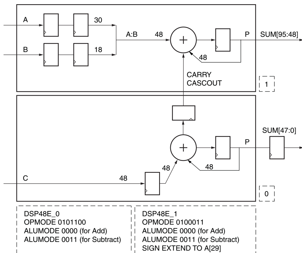
Figure 4-22: 96-Bit Accumulator
