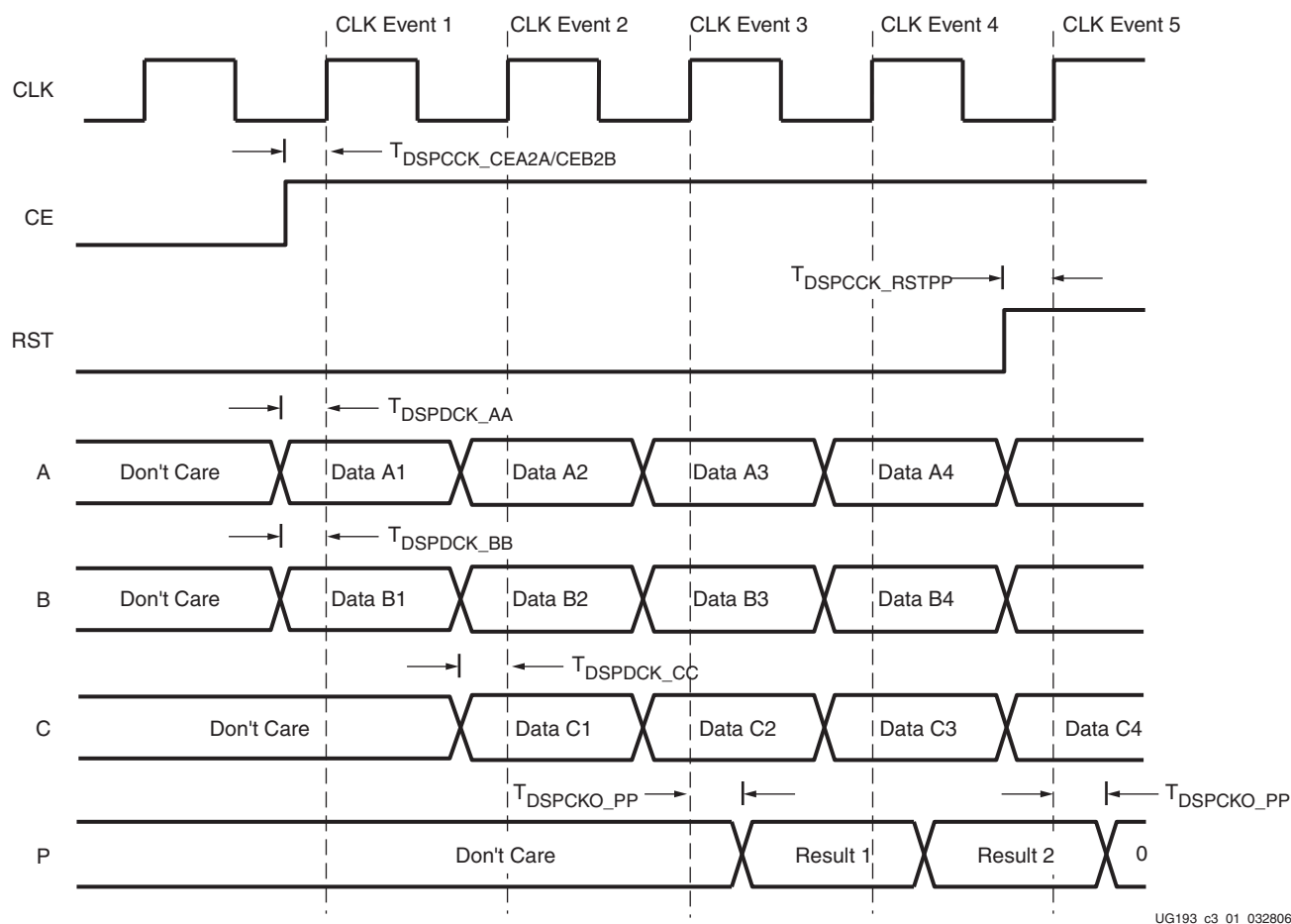
Figure 3-1: DSP48E Timing Diagram
