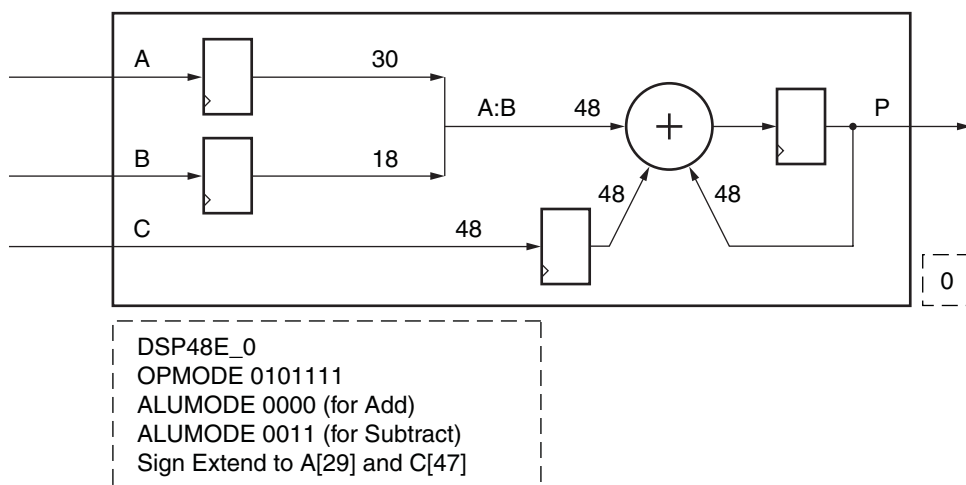
Figure 4-20: 48-Bit Dynamic Add/Sub Accumulator
