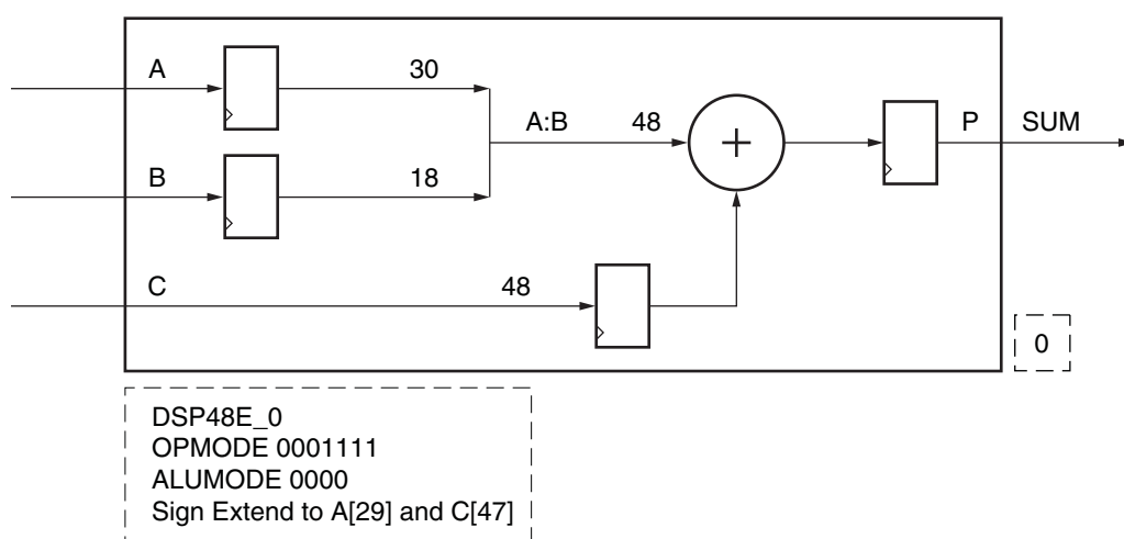
Figure 4-9: Two Input 48-Bit Addition
