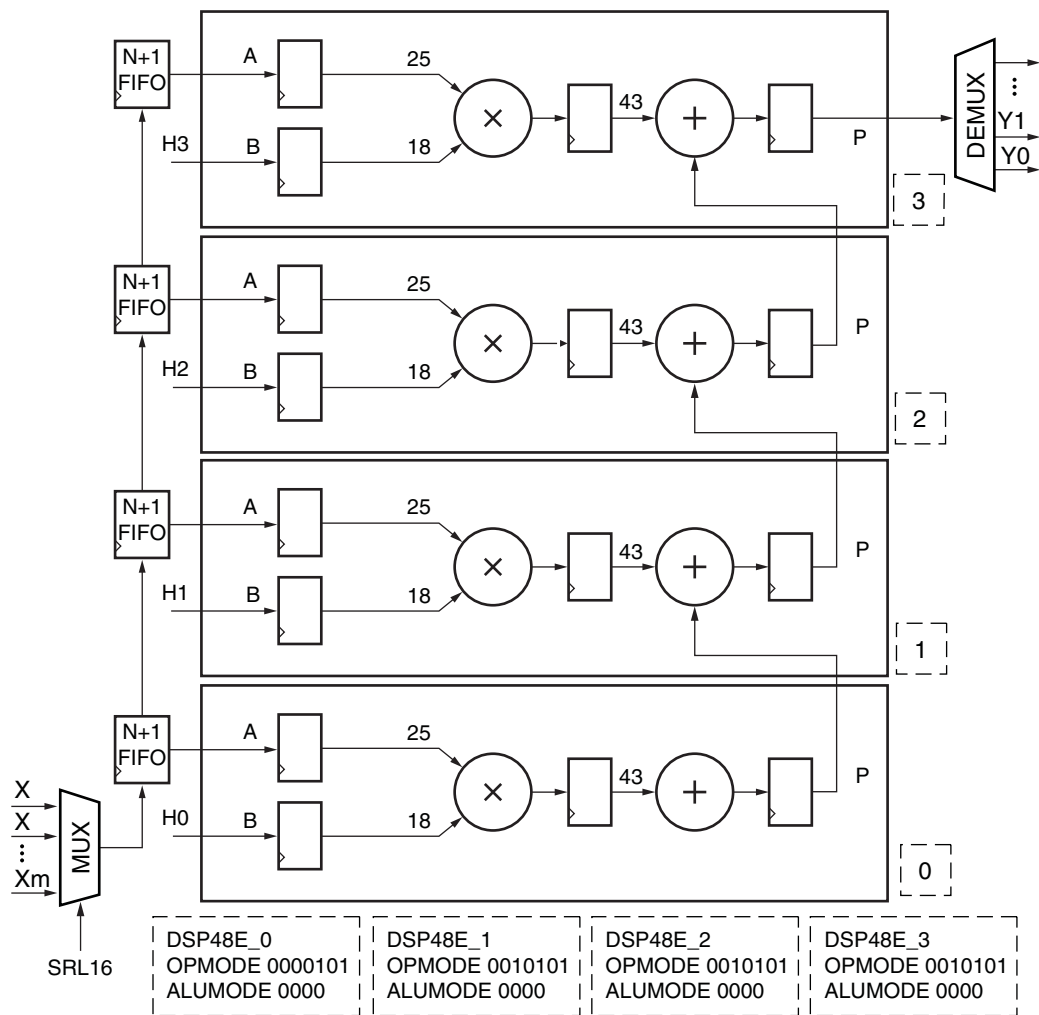
Figure 4-32: Multichannel FIR Filter
