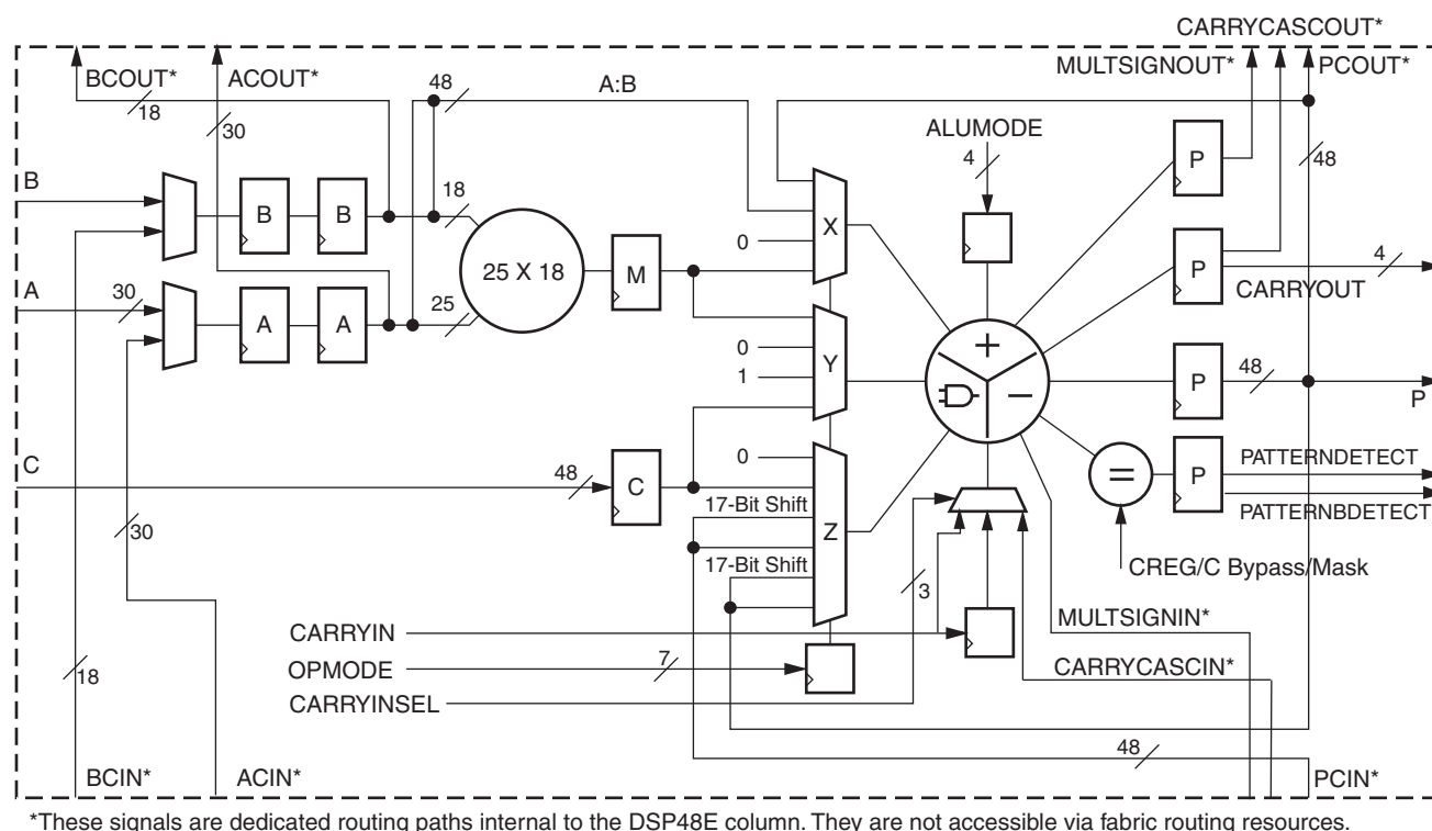
Figure 1-1: Virtex-5 FPGA DSP48E Slice
