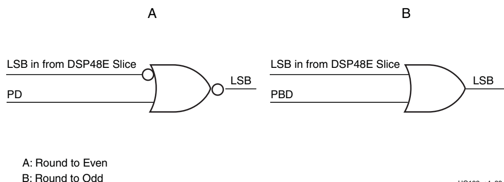
Figure 4-40: A: Round to Even and B: Round to Odd
