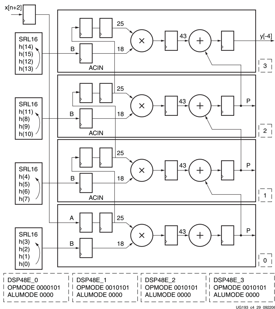
Figure 4-30: 16-Tap 1:4 Interpolator
