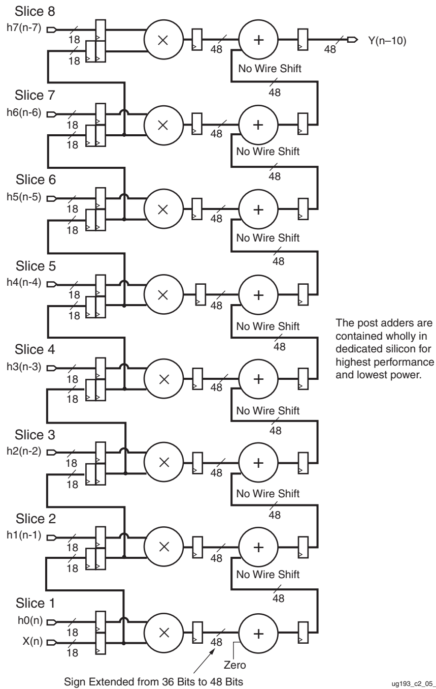
Figure 2-5: Adder Cascade
