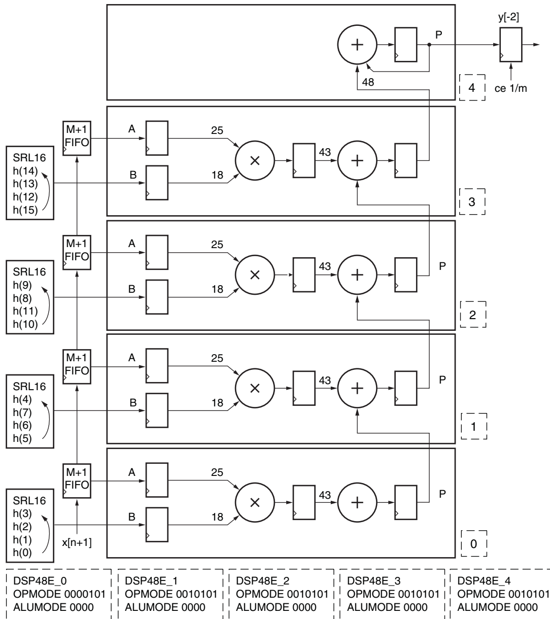
Figure 4-31: 16-Tap 1:4 Decimator
