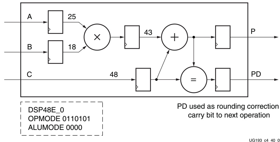
Figure 4-41: Convergent Rounding: Carry Correction
