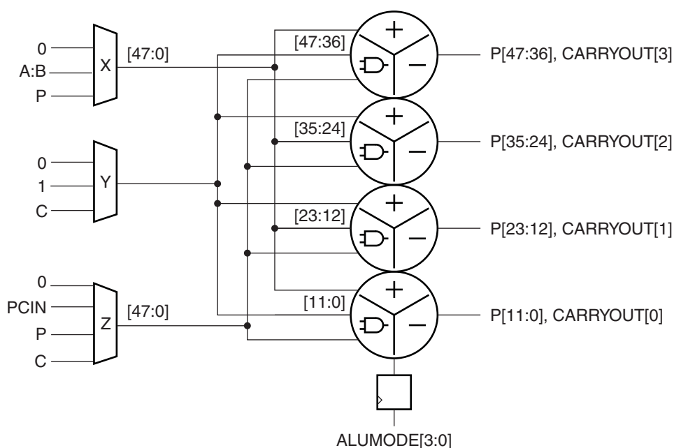
Figure 1-15: Four 12-Bit SIMD Adder Configuration
