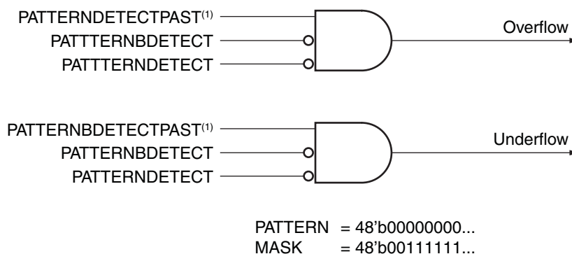
Figure 1-17: Overflow/Underflow Logic in Pattern Detect
