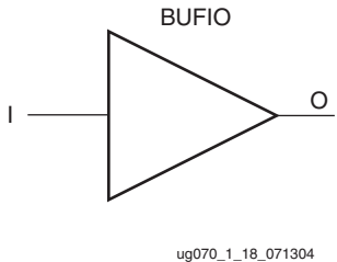
Figure 1-18: BUFIO Primitive
