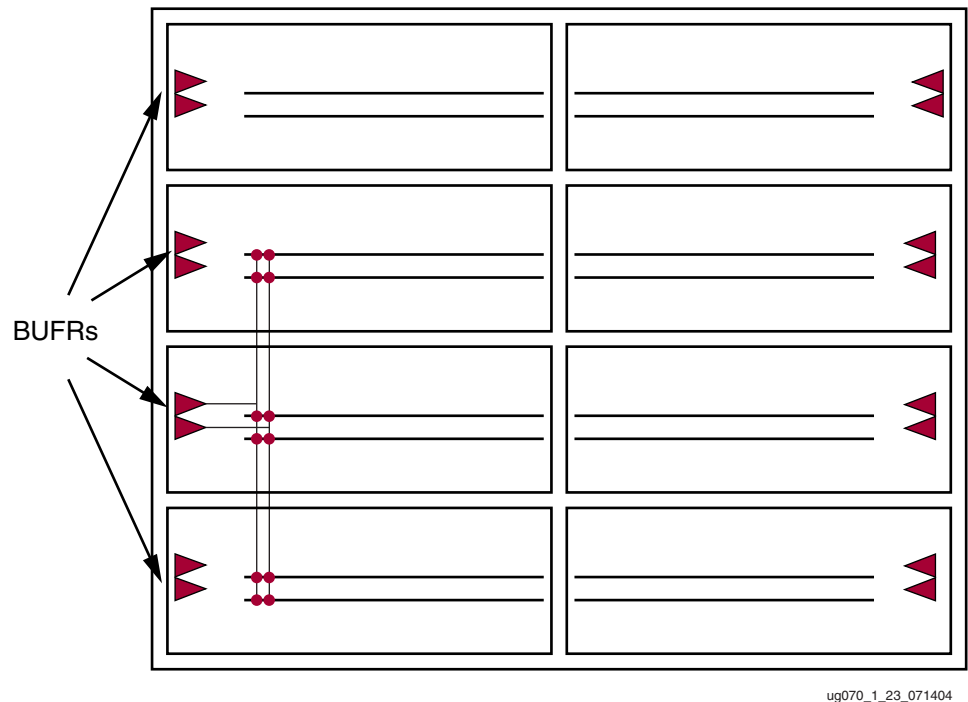
Figure 1-23: BUFR Driving Multiple Regions
