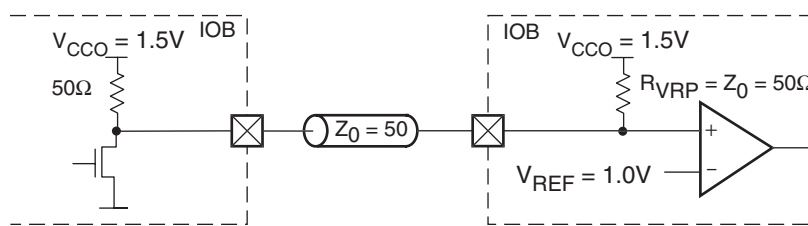
Figure 6-38: GTLP_DCI Internal Parallel Driver and Receiver Termination
