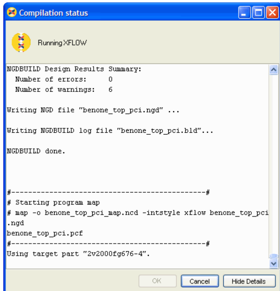
Figure 4-9: Compilation Status
