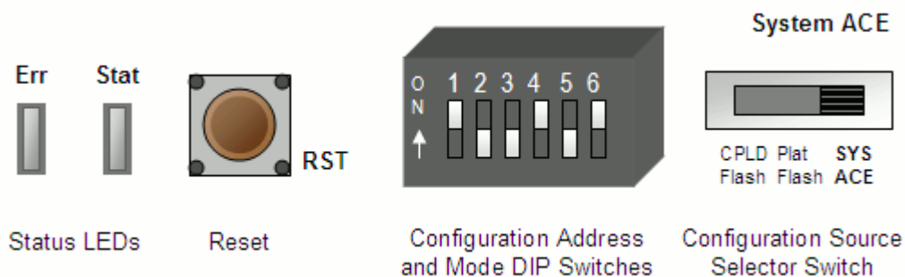
Figure 4-13: On-Board Settings
