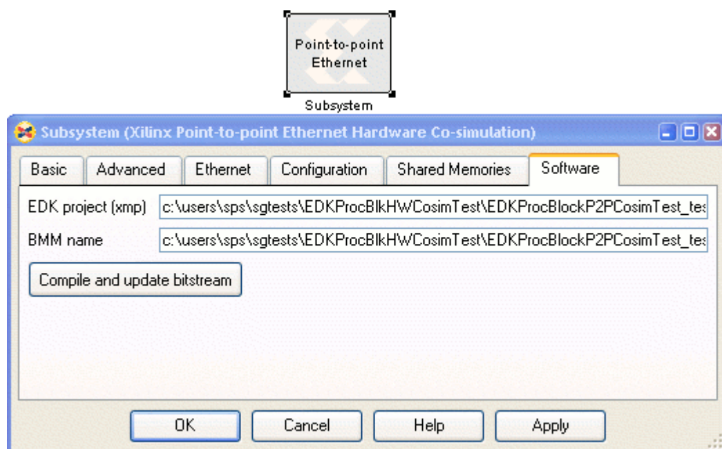
Figure 3-8: Software Tab
