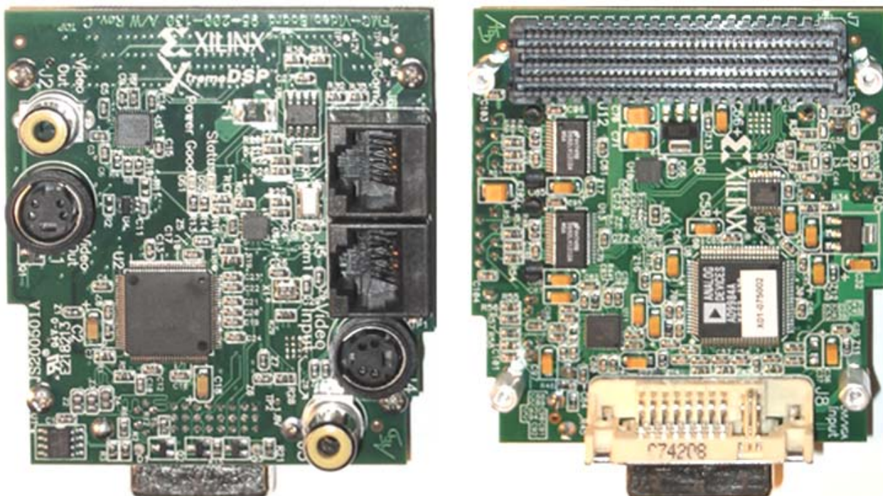
Figure 1-4: FMC-Video Top (Left), Bottom (Right)
