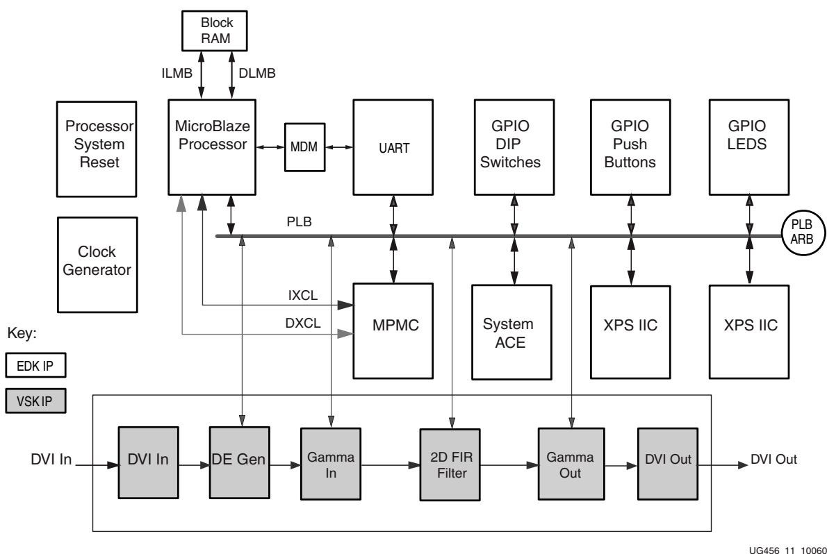
Figure 3-3: DVI Pass-Through Demo: System-Level Block Diagram
