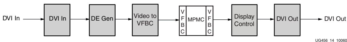
Figure 3-4: DVI Frame Buffer: Video Pipeline
