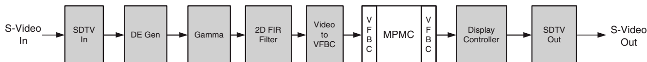
Figure 3-10: S-Video Frame Buffer: Video Pipeline
