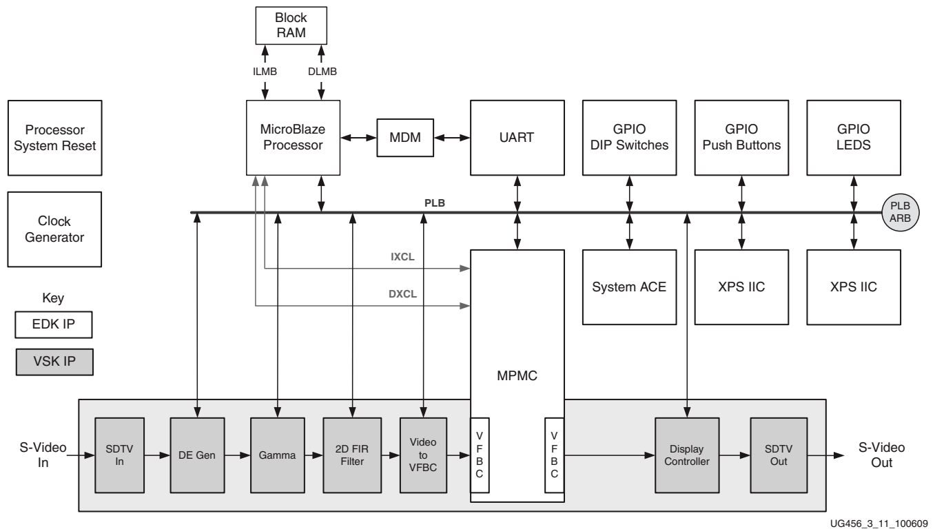
Figure 3-11: S-Video Frame Buffer Demo
