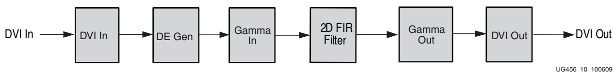
Figure 3-2: DVI Pass-Through: Video Pipeline
