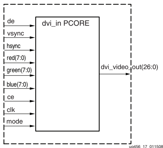
Figure B-2: dvi_in PCORE
