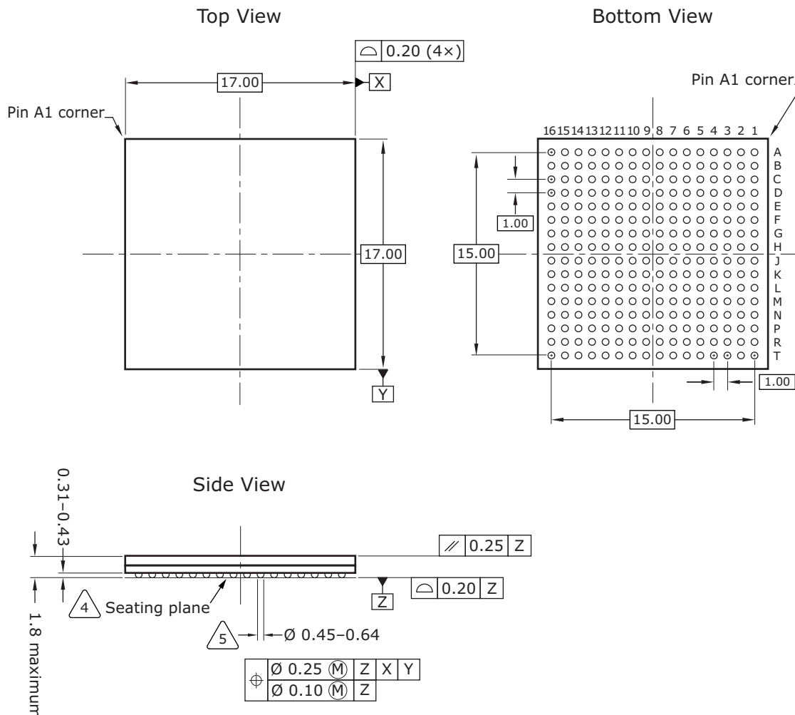
Figure 134 • Package Drawing
