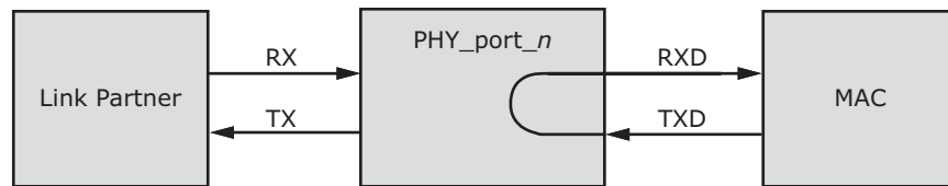
Figure 109 • Near-End Loopback Diagram
