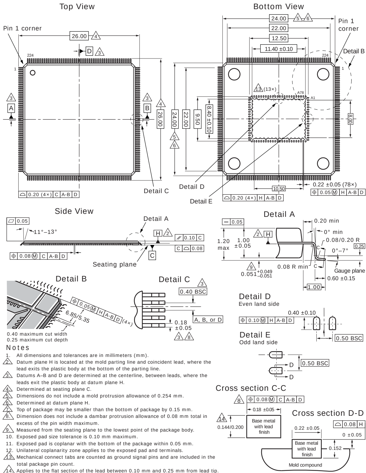
Figure 30 • Package Drawing
