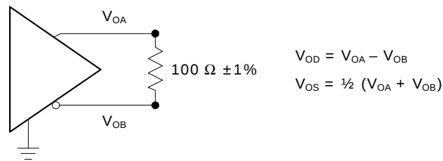
Figure 27 • SGMII DC Transmit Test Circuit
