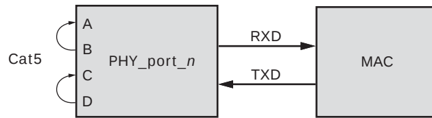
Figure 23 • Connector Loopback Diagram
