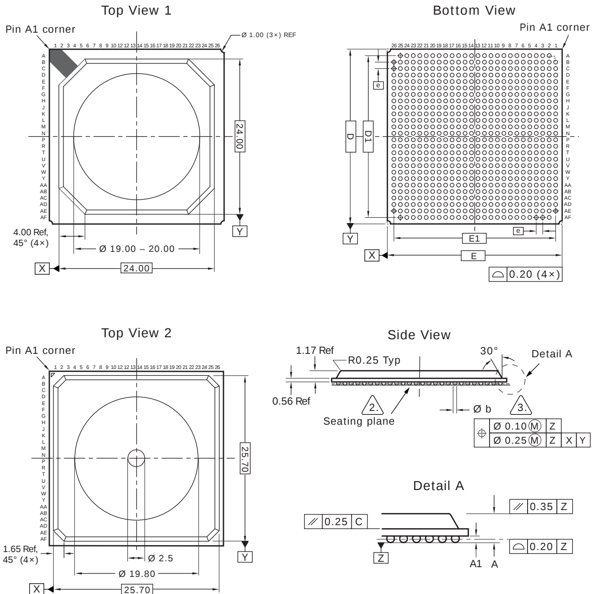
Figure 40 • Package Drawing
