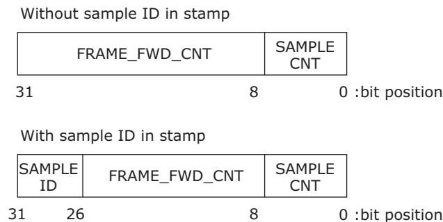
Figure 43 • sFlow Stamp Format in FCS
