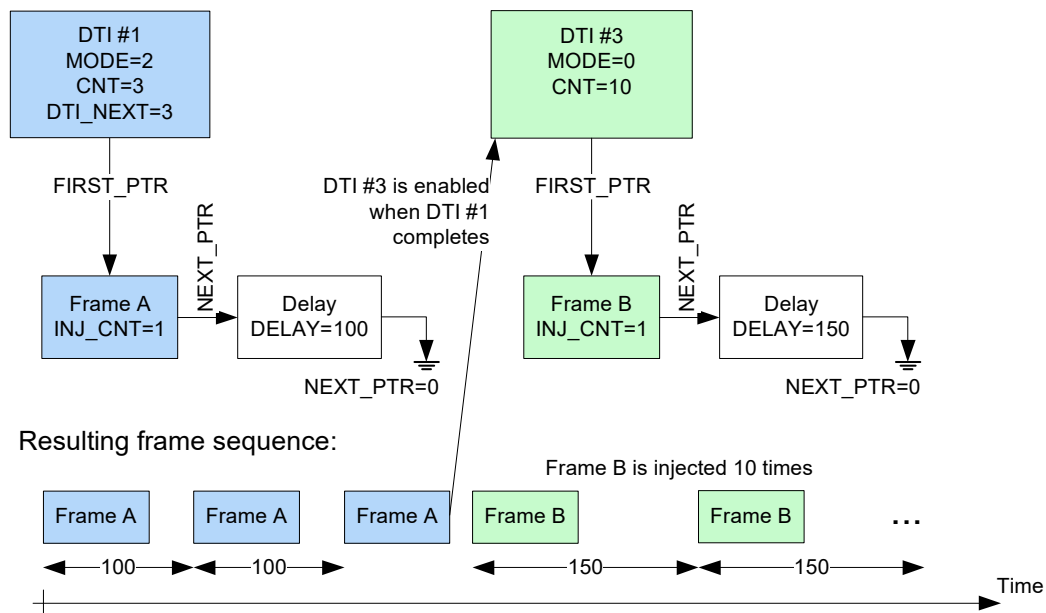
Figure 67 • DTI Concatenation
