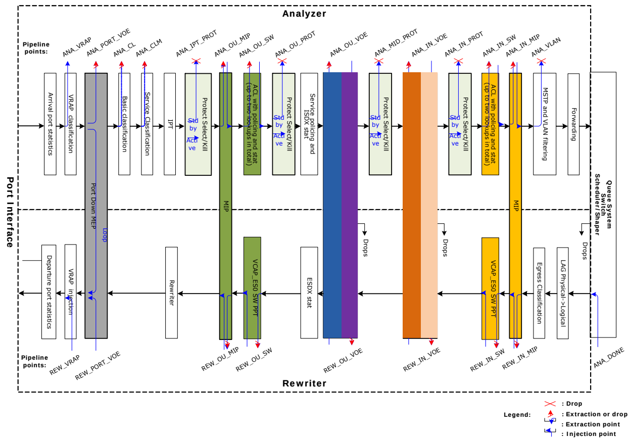
Figure 13 • Processing Flow
