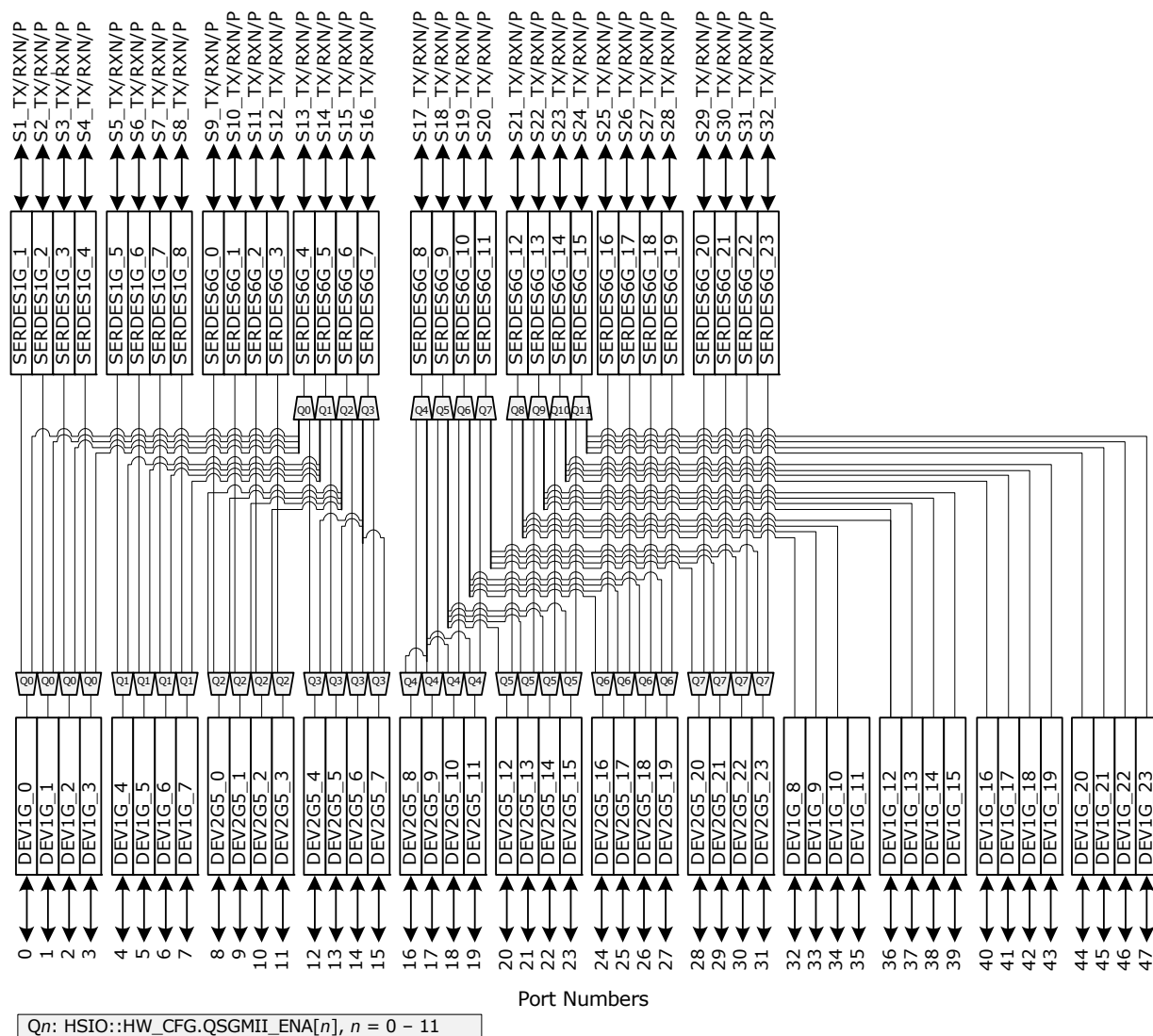
Figure 8 • QSGMII Muxing
