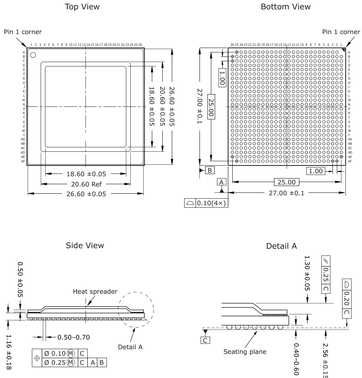
Figure 149 • Package Drawing
