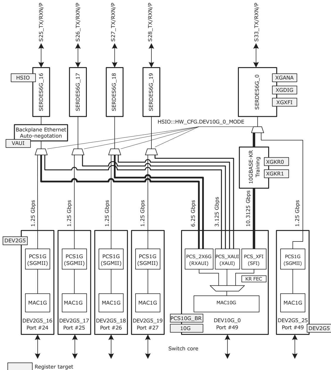
Figure 9 • 10G Muxing
