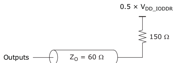
Figure 134 • Test Load Circuit for DDR3 Outputs
