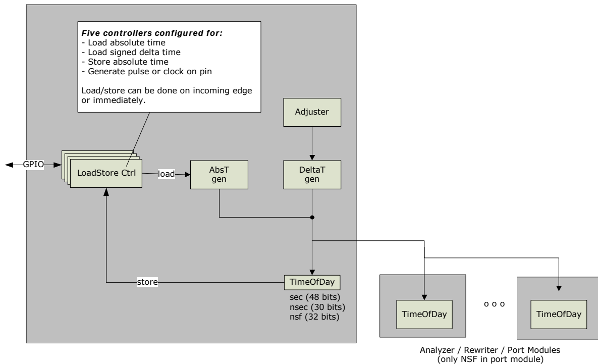
Figure 78 • Timing Distribution
