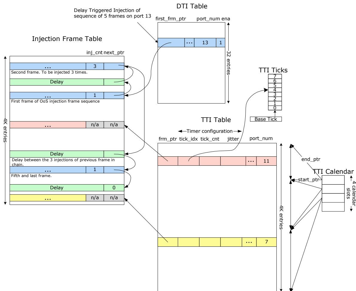
Figure 62 • Injection Tables
