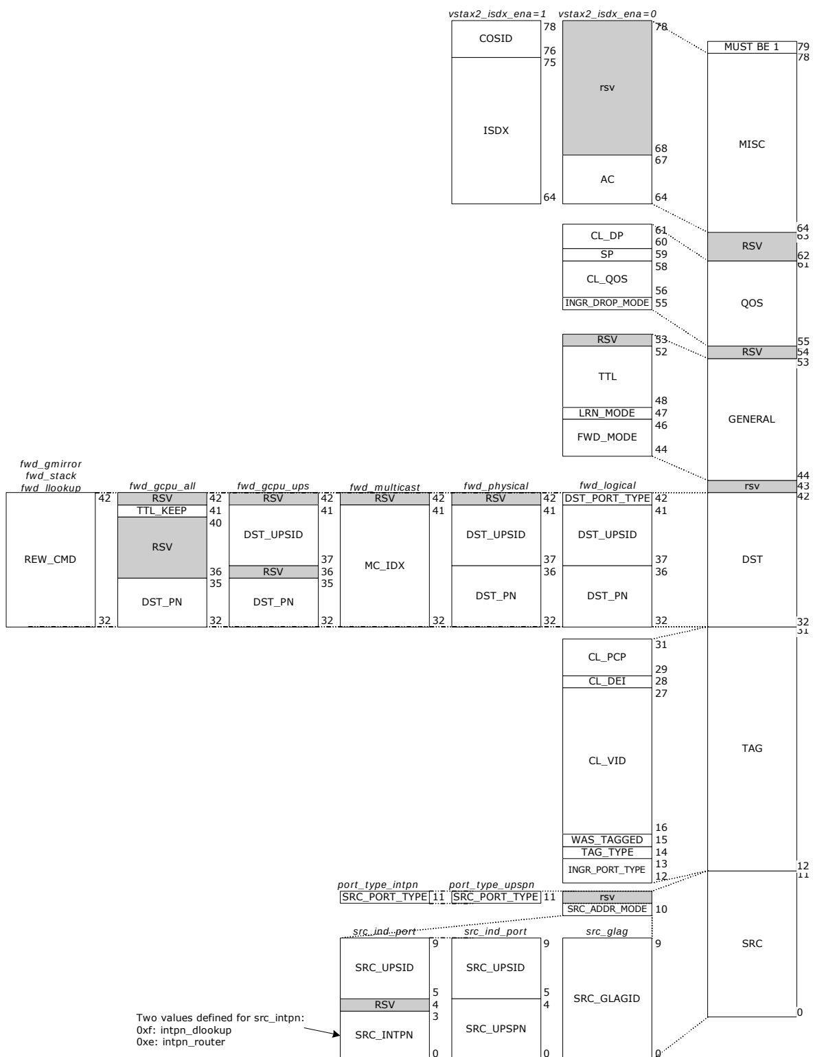
Figure 7 • VStaX Header Layout
