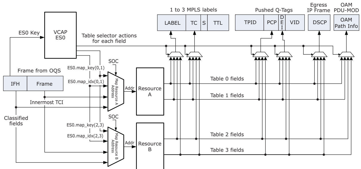
Figure 71 • Mapping Tables
