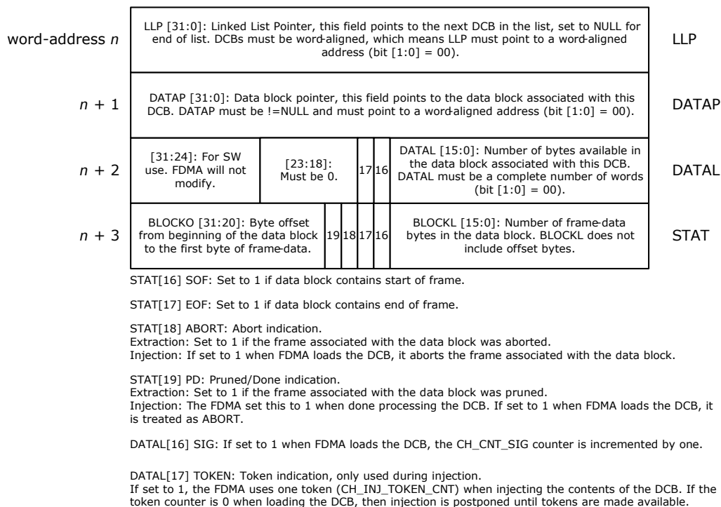
Figure 99 • FDMA DCB Layout
