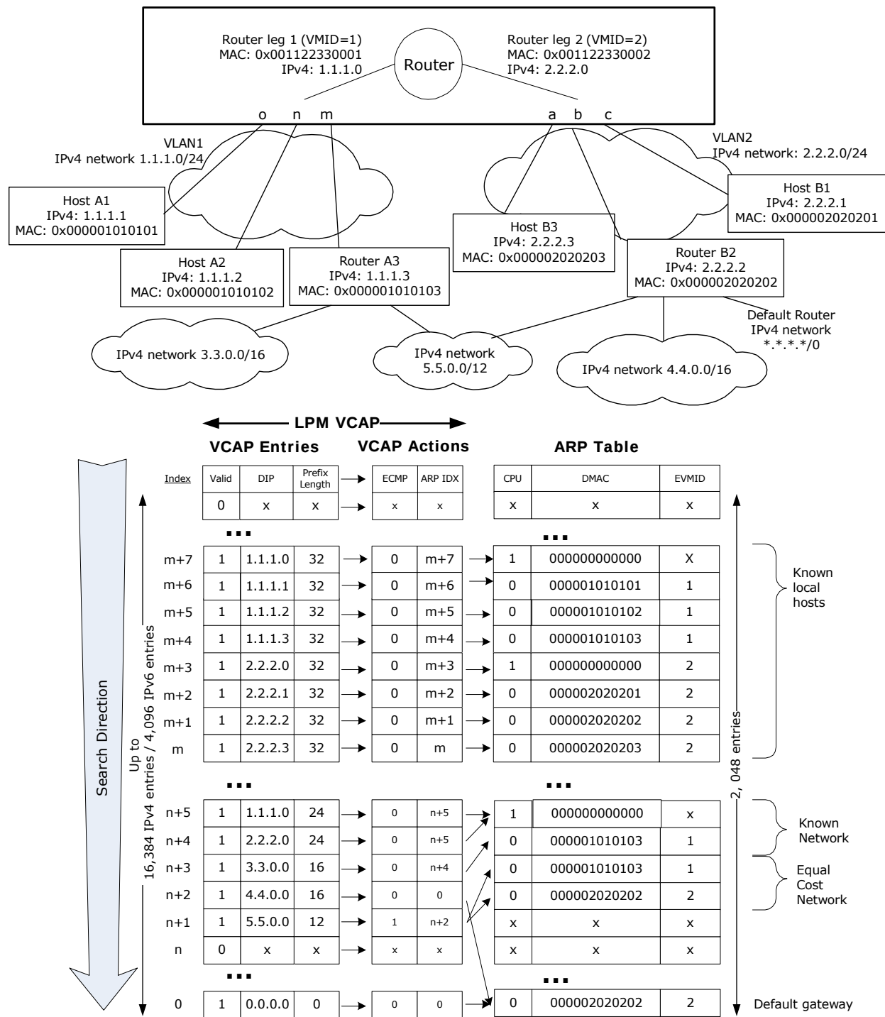
Figure 26 • IP Unicast Routing Example
