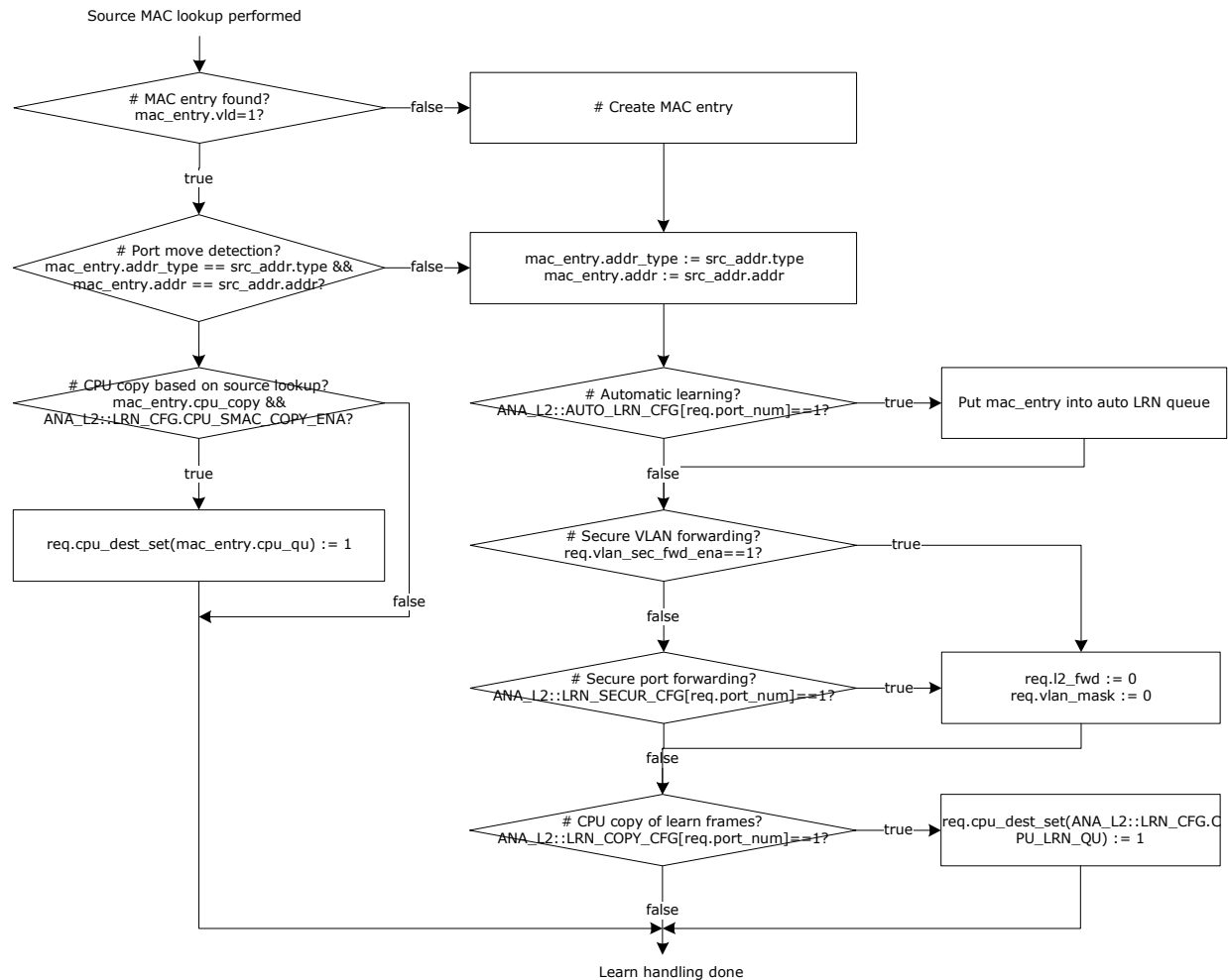
Figure 31 • Source Check
