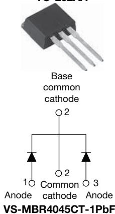
TO-262AA
