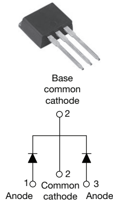
TO-262
