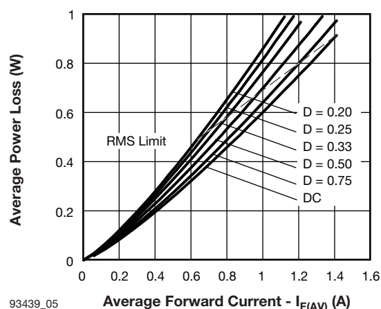
93439_05 Average Forward Current - I F(AV) (A) Fig. 5 - Forward Power Loss Characteristics
