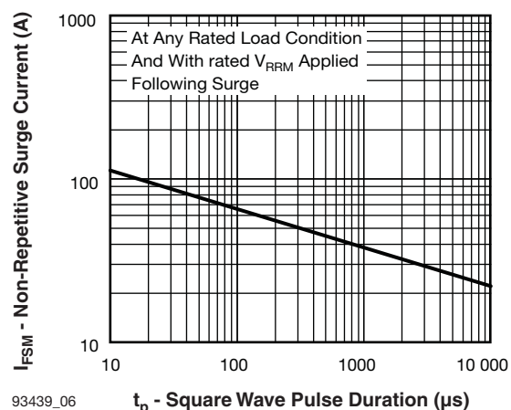
93439_06 t p - Square Wave Pulse Duration (μs) Fig. 6 - Maximum Non-Repetitive Surge Current
