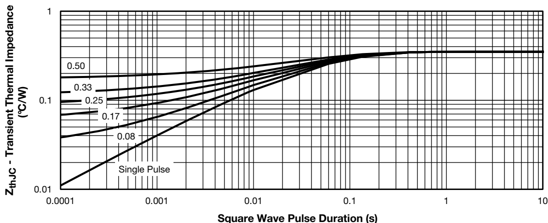
Fig. 9 - Thermal Impedance Z_{th,IG} Characteristics
