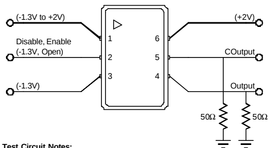
Figure 2. 3.3V Test Circuit
