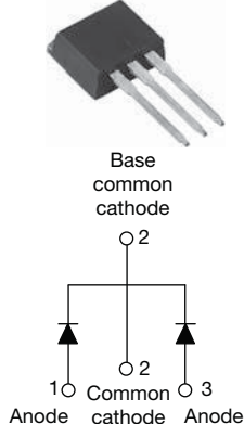
VS-30CTQ...-1PbF
